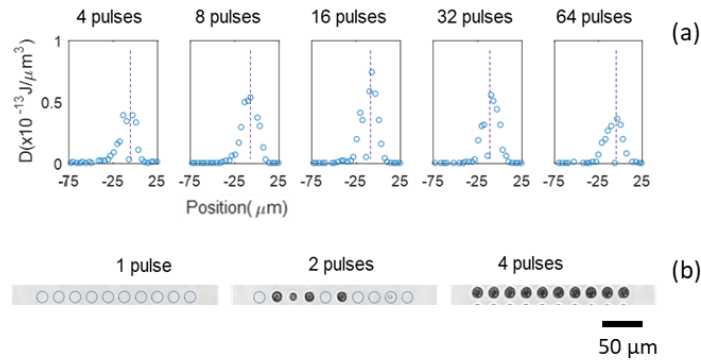
Fig.1. Accumulating energy density with pulse trains. (a) Estimated absorbed energy densities (peak) along the propagation distance (geometrical focus at zero-position) with trains of femtosecond pulses (5.6 THz) focused with NA=0.45 (b) Top-view infrared images of modifications produced with trains of 4-ps pulses at focused (NA=0.85) 300 \mu\text{m} below the surface. All irradiation energies are the same (2.1 \mu\text{J}/\text{train} ) repeated 10 times for direct comparisons of damage probabilities.
