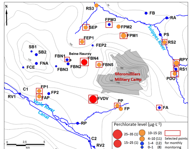
Figure 2. Perchlorate levels in waters in June 2017 and selected sampling points for the monthly monitoring.
