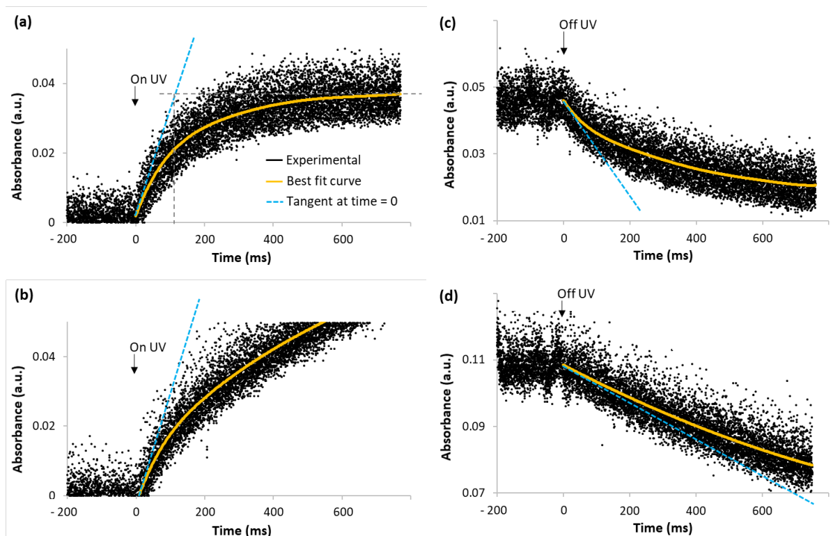
Figure 5. QCL beam absorbance at 1360\text{ cm}^{-1} vs. time over \text{TiO}_2 P25 during a UV on-off cycle (UV on: a-b, UV off: c-d) under flowing methanol at 25\text{ }^\circ\text{C} and atmospheric pressure in the presence (a and c) or absence (b and d) of oxygen. Conditions: flow = 30\text{ mL/min} ; 0.1\text{ vol.}\% of methanol in argon, with 20\text{ vol.}\% of oxygen if present; Hg-Xe lamp ( 200\text{ W} ); I_0 \approx 200\text{ mW/cm}^2 . In (a-b), time = 0 corresponds to the moment when the shutter in-between the lamp and the UV-light guide directed to the IR cell was opened to irradiate the sample. During the preceding 200\text{ ms} , the sample was already under flowing methanol (with oxygen in a, without oxygen in b) but still in the dark. In (c-d), time = 0 corresponds to the moment when the shutter was closed again, still under the same flow as in (a-b). The times to open and close the shutter were around 6.5\text{ ms} and 3.2\text{ ms} , respectively.
