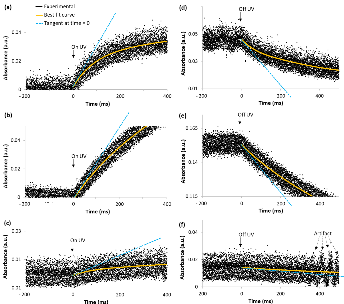
Figure 2. QCL beam absorbance at 1360\text{ cm}^{-1} vs. time over \text{TiO}_2 P25 (a and d), \text{TiO}_2 CA (b and e) and \text{TiO}_2 HA (c and f) during the first UV on-off cycle (UV on: a-b-c, UV off: d-e-f) under reaction flow at 25\text{ }^\circ\text{C} and atmospheric pressure. Conditions: flow = 30\text{ mL/min} ; 0.1 and 20 vol.% of methanol and oxygen in argon, respectively; Hg-Xe lamp ( 200\text{ W} ); I_0 \approx 200\text{ mW/cm}^2 . In (a-b-c), time = 0 corresponds to the moment when the shutter in-between the lamp and the UV-light guide directed to the IR cell was opened to irradiate the sample. During the preceding 200 ms, the sample was already under reaction flow but still in the dark. In (d-e-f), time = 0 corresponds to the moment when the shutter was closed again, still under reaction flow. The fall times to open and to close the shutter were around 6.5 ms and 3.2 ms, respectively, with a minimum pulse width of 13 ms.
