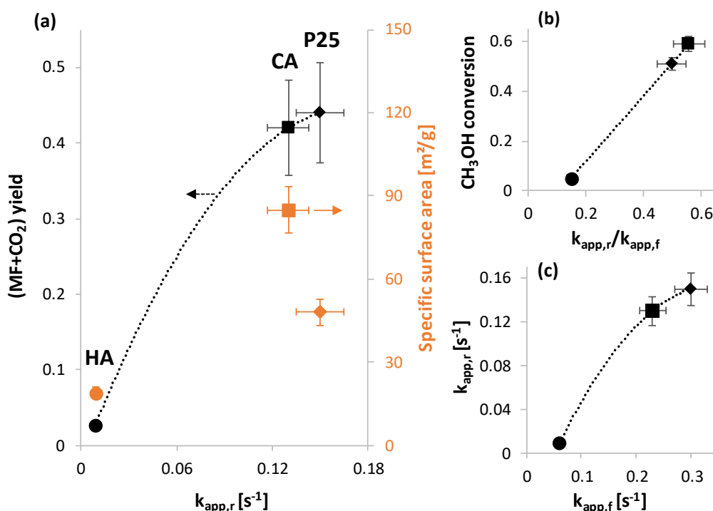
Figure 3. (a) Evolution of the (MF+CO 2 ) yield vs. the k_{app,r} of formate species over TiO 2 HA (circle), CA (square) and P25 (losange) (the specific surface area of the three photocatalysts is also shown, as a reference). (b) Methanol conversion vs. k_{app,r}/k_{app,f} ratio of formate species. (c) k_{app,r} vs. k_{app,f} of formate species. Conditions: reaction flow = 30 mL/min containing 0.1 and 20 vol.% of methanol and oxygen in argon, respectively; Hg-Xe lamp (200 W) filtered at \lambda = 365 nm; I_0(365nm) \approx 15 mW/cm 2 .
