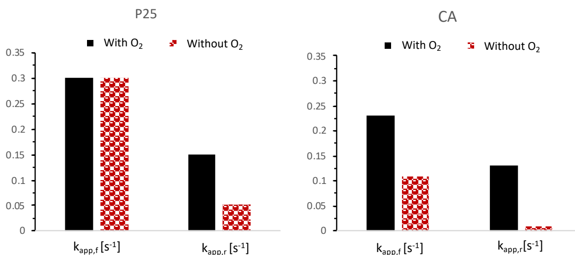
Figure 4. For TiO 2 P25 and CA: apparent rate constants for the formation and reaction of formate species ( k_{app,f} and k_{app,r} , respectively) at 25 °C and atmospheric pressure in the absence vs. presence of oxygen in the reaction flow. Conditions: flow = 30 mL/min; 0.1 vol.% of methanol in argon, with 20 vol.% of oxygen if present; Hg-Xe lamp (200 W); I_0 \approx 200 mW/cm 2 .
