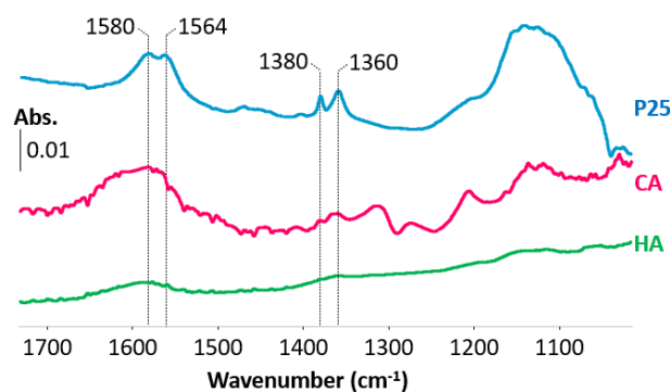
Figure 1. Operando FT-IR spectra at steady state of TiO 2 P25, TiO 2 CA and TiO 2 HA upon photooxidation of methanol at 25 °C and atmospheric pressure, shown after subtraction of the initial spectrum recorded after dehydration pre-treatment under flowing methanol before UV irradiation. Conditions: flow = 30 mL/min; 0.1 and 20 vol.% of methanol and oxygen in argon, respectively; Hg-Xe lamp (200 W) filtered at \lambda = 365 nm; I_{0(365\text{nm})} \approx 15 mW/cm 2 . “Abs.” means absorbance, and is expressed in arbitrary units.
