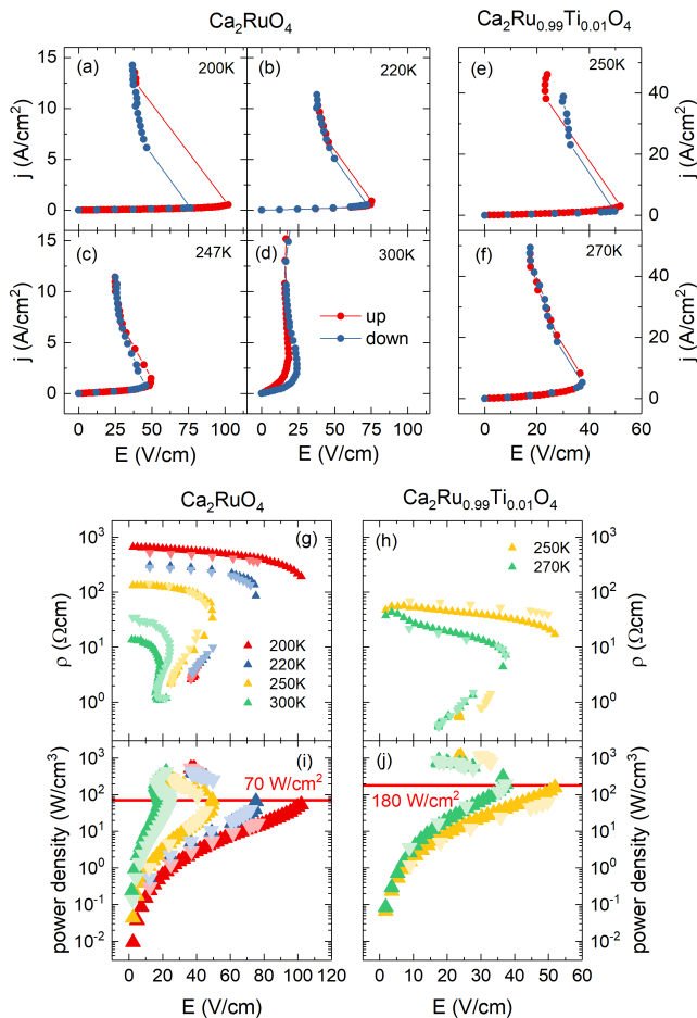
FIG. 2. Switching characteristics of pure and 1% Ti-substituted \text{Ca}_2\text{RuO}_4 in dependency of temperature. (a)-(f) Characteristic j - E curves display the current-induced phase transition in a voltage controlled setup (The electric field has been corrected for the circuit resistance effects). Here red coloring denotes data taken for ramping the voltage up and blue for ramping down. (g)-(h) The calculated resistivities from the two-point measurements above show a clear drop at a temperature dependent critical electric field. (i) and (j) represent the corresponding power densities in the j - E characteristic. The threshold power density, at which the switching occurs, is constant for all measured temperatures. Dark coloring is used for the up direction, light coloring for the down direction.
