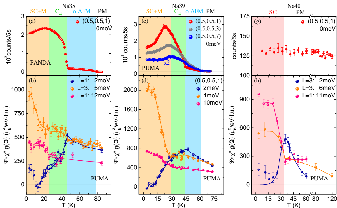
Figure 5. Temperature dependence of the elastic and inelastic response. (a) The temperature dependent scattering of the (0.5, 0.5, 1) magnetic Bragg peak of Na35 shows the three phase transitions, data taken from [29] and binned within 1 K. (b) Inelastic response of Na35 displays a peak for 2 meV at T_{\text{reo}} , while the intensity uptake at 5 meV and 12 meV corresponds to the formation of the resonance mode. (c) Elastic response of Na39 determined at the (0.5, 0.5, L) positions that sense c and a polarized moments differently [45], data taken from [47]. (d) Inelastic response of Na39 at (0.5, 0.5, 1) showing for 2 meV a maximum at T_{\text{reo}} and a suppression in the SC phase. The emergence of the SRM's result in increasing intensities at 4 meV and 10 meV below T_c . (e) The constant elastic scattering at the (0.5, 0.5, 1) magnetic Bragg-position for Na40 shows the absence of magnetic ordering down to the lowest temperatures, data taken from [47]. (f) Inelastic response of Na40 showing a maximum for 2 meV at T_c and an intensity uptake due to the SRM formation at 6 meV and 11 meV, respectively. All lines are guides to the eye and the colored backgrounds correspond to the SC, C_4 and o-AFM phases.
