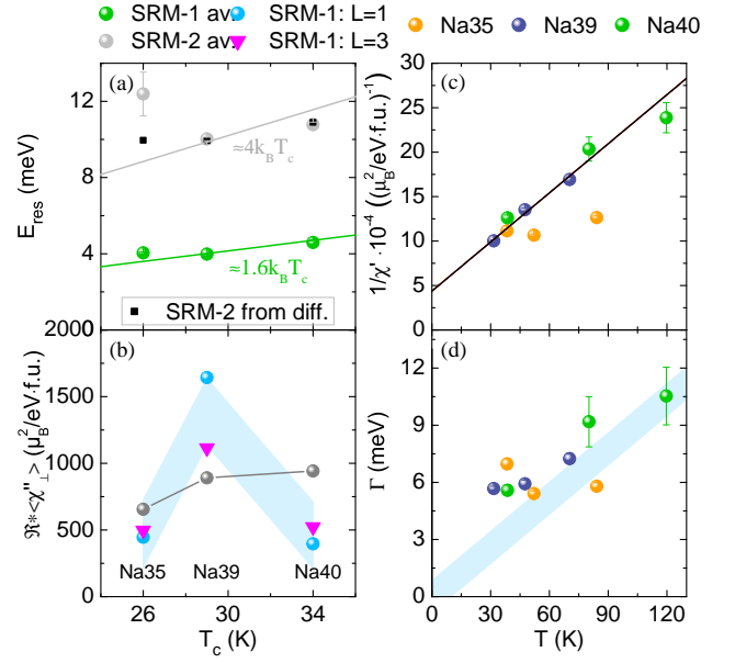
Figure 4. Energies and amplitudes of magnetic scattering. Parameters describing the magnetic response obtained from the spectra and difference spectra. (a) and (b) show the energies and the amplitudes of the SRM-1 and SRM-2 log-normal functions plotted against the T_c of the three samples studied. For the high-energy SRM-2 we include the value obtained from fitting the intensity differences shown in Fig. 3 (black squares). (c) and (d) resume the single-relaxor parameters describing the normal-state response traced against the temperature. One recognizes that Na39 and Na40 behave very similarly concerning both the amplitude and the characteristic energies, while the response of Na35 is determined by the stronger static AFM order. The linear fit in (c) corresponds to a Curie-Weiss law, and the blue bar in (d) denotes the Planck scaling \Gamma = k_B T .
