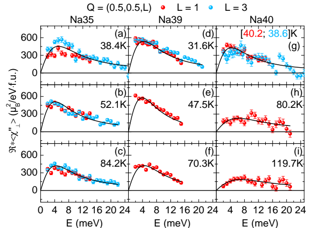
Figure 2. Magnetic excitations at the AFM Bragg positions in the normal state (a)-(i) Magnetic scattering presented in absolute units for the three samples recorded at (0.5, 0.5, 1) and (0.5, 0.5, 3) at various temperatures. The NS response is described by a single relaxor function convoluted with the instrumental resolution.
