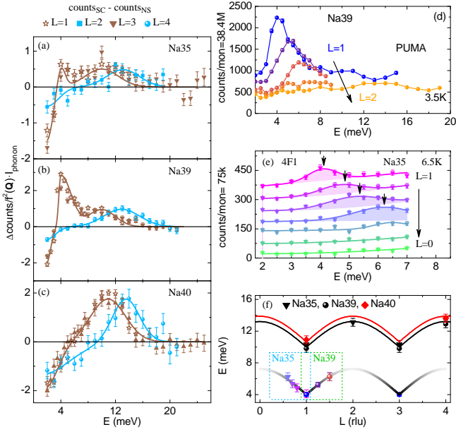
Figure 3. Dispersion of the resonance modes. (a)-(c) Normalized intensity difference of the SC state and NS at odd and even L -values for Na35, Na39 and Na40, respectively. Solid lines are (asymmetric, i.e. different widths above and below the peak) Gaussians peaking at different energies for odd respectively even L -values. Data in the SC state was taken at 3.5 K, and data in the NS at 38 and 32 K for Na35 and Na39, respectively, and at 39 and 40 K for L=1 and 3 with Na40. (d) Lower part of the split spin resonance mode for 1 \leq L \leq 2 of Na39 displays a dispersion to higher energies and a reduction in intensity. (e) Same as in (d) but for Na35 at 0 \leq L \leq 1 . (f) Fit of the dispersion as described in the main text in which the data points of Na35 and Na39 were combined. Disregarding the color, all triangular symbols belong to Na35, while all spherical symbols belong to Na39.
