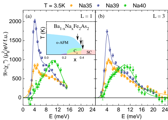
Figure 1. Spin resonance modes in the superconducting phases. INS spectra obtained at the AFM Bragg positions (0.5, 0.5, L) with L=1, 3 for the three samples studied. Data were corrected for background, for the Bose and form factors and normalized to absolute units, see methods section. The spectra were fitted with two log-normal functions corresponding to the two SRM's at 4 and 8-10meV. The inset indicates the location in the phase diagram of \text{Ba}_{1-x}\text{Na}_x\text{Fe}_2\text{As}_2 for the three samples studied.
