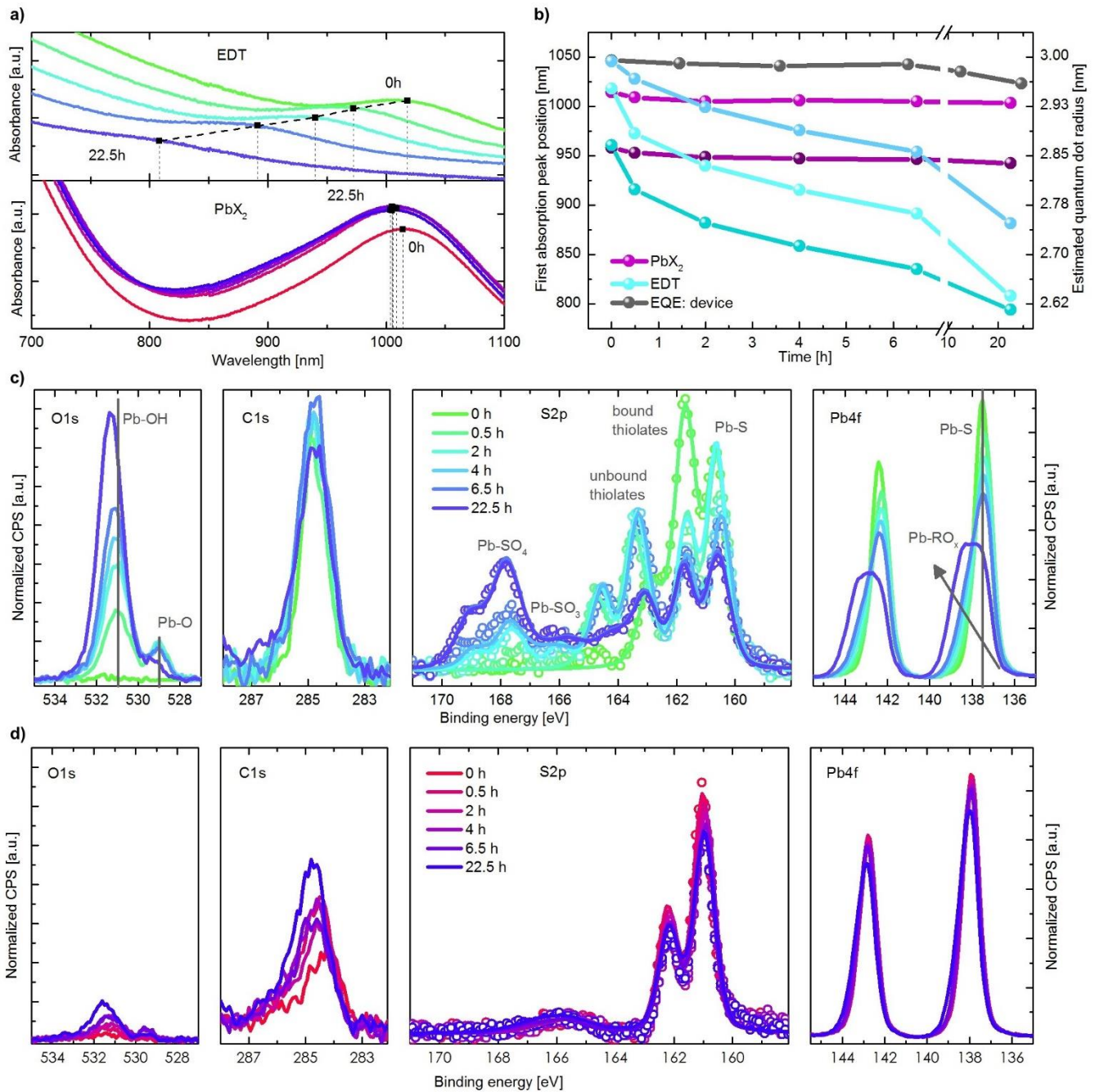
Figure 3. Initial QDs size dependence and ligand controlled degradation behaviour. Upper row from left to right: Absorption measurements of EDT and PbX 2 covered QDs for different time steps in an oxygen atmosphere. Extracted position of the first absorption peak maximum for different ligands and initial dot sizes, also including positions from an EQE measurement of a device. Middle row: XPS data of EDT-PbS
