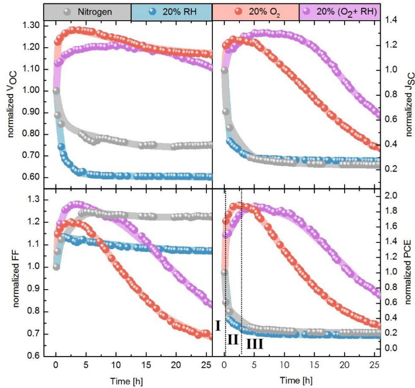
Figure 2. Evolution of photovoltaic parameters under different atmospheres. From left to right, the panels show the normalized V_{oc} , J_{sc} , FF and PCE. The lines behind the data points are meant as a guide for the eye. In the PCE panel, the three phases of degradation under oxygen (I, II, and III) are defined. The first data point of each curve is always measured in nitrogen only. The gas flow is started after the first measurement.
