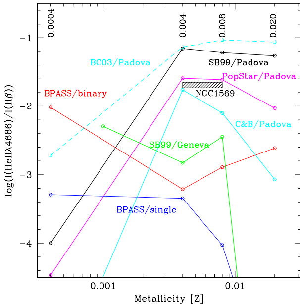
Figure 10. Maximum values of the nebular I(He II \lambda 4686 )/I(H \beta ) ratio (points joined by lines) reached as a function of the abundance for the SSP models indicated close to each curve. The observed value for NGC 1569 is indicated, where the range in metallicity takes into account 10–30% depletion of oxygen into dust grains ( Gutkin, Charlot & Bruzual 2016 ). The observed values are in agreement with the highest values of model I(He II \lambda 4686 )/I(H \beta ) ratio, that happens between Z=0.004 and Z=0.008 for new (C&B/Padova) as well as old Padova (SB99/Padova, PopStar/Padova) models.
