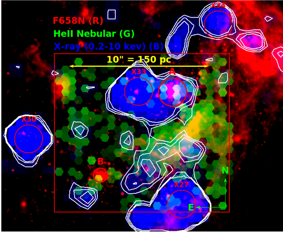
Figure 11. X-ray emission map from the Chandra/ACIS image (0.2–10 keV band) from Sánchez-Cruces et al. (2015) in blue is superposed on the He II nebular map in green and F658N ( H\alpha +continuum) in red. The contours show the X-ray emission at 3 levels ( 3\sigma , 3.5\sigma and 4\sigma above the background) to help see the position of the faint X-ray diffuse emission with respect to the He II \lambda 4686 nebular emission. Most of the X-ray emission within the MEGARA FoV (red square) originates in two hard X-ray point sources (X27 and X33), which are marked by red circles. The diffuse X-ray emission coincides with part of the He II \lambda 4686 nebular emission. However, there is no X-ray emission at the brightest zone of the nebular He II \lambda 4686 emission.
