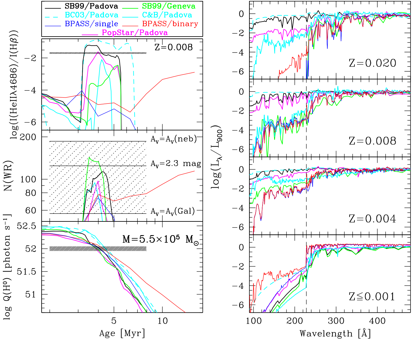
Figure 9. (Left panels) Comparison of observed quantities in NGC 1569 with Population Synthesis models. The plotted observed quantities (horizontal hatched areas) are the ratio of integrated nebular He II \lambda 4686 line flux to that of H \beta line (top-left), number of WR stars in SSC-A (middle-left) and the rate of hydrogen ionizing photons determined from the integrated H \beta flux (bottom-left). Results from 7 different population synthesis models are shown, which are identified in a box above the plots (see text and Table 1 for details of these models). Models that use Padova evolutionary tracks are able to reproduce the observed values for a cluster of mass =5.5 \times 10^5 M_{\odot} at an age of 4 Myr. All models use Kroupa IMF at Z=0.008 , which is the metallicity closest to that of NGC 1569 available in all the codes. (right panels) Spectral shape near the He + ionizing edge (228 Å) at the 4 indicated metallicities during the WR phase. Spectra are shown normalised to their flux at 900 Å wavelength. All spectra show a jump blueward of 228 Å at the lowest plotted metallicity. However, at higher metallicities the spectral shapes blueward of 228 Å for the plotted models do not coincide, with the spectra being harder in models incorporating Padova tracks as compared to those obtained using other tracks.
