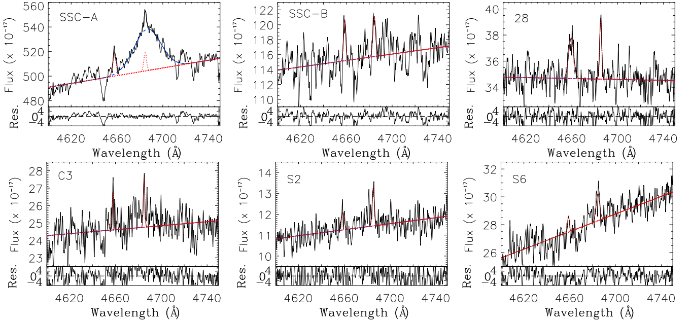
Figure 4. Multi-fibre summed spectra around the BB of SSC-A and other cluster and stellar sources in the FoV of MEGARA/IFU. No WR stars are detected in clusters SSC-B and 28. Star cluster C3 and stellar sources S2 and S6, where the presence of WR stars have been previously reported from the analysis of the HST F469N-band narrow-band images, only show nebular lines in our spectra. The fluxes are plotted in units of 10^{-17} erg cm ^{-2} s ^{-1} Å ^{-1} , and the bottom panel of each plot shows the residual flux in the same units.
