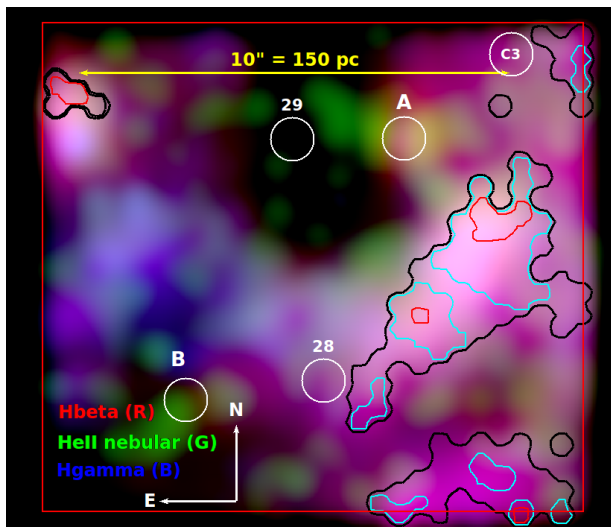
Figure 7. Extinction contours superposed on the MEGARA RGB nebular images. Smoothed images in H\beta , He\ II\ \lambda 4686 and H\gamma are used as red, green and blue components, respectively. The contours corresponding to A_V=1.6 , 2.6 and 3.6 mag are shown in black, cyan and red colours, respectively. The noise in the measured fluxes in individual fiber spectra did not allow the determination of reliable A_V values outside the black contours, though emission is seen in this smoothed image. Known sources in the FoV are labelled. The zone with the highest He\ II\ \lambda 4686 nebular emission (south-west of SSC-A) is also the zone with the highest A_V . The nebular emission follows a semi-circular arc of \sim 150 pc diameter.
