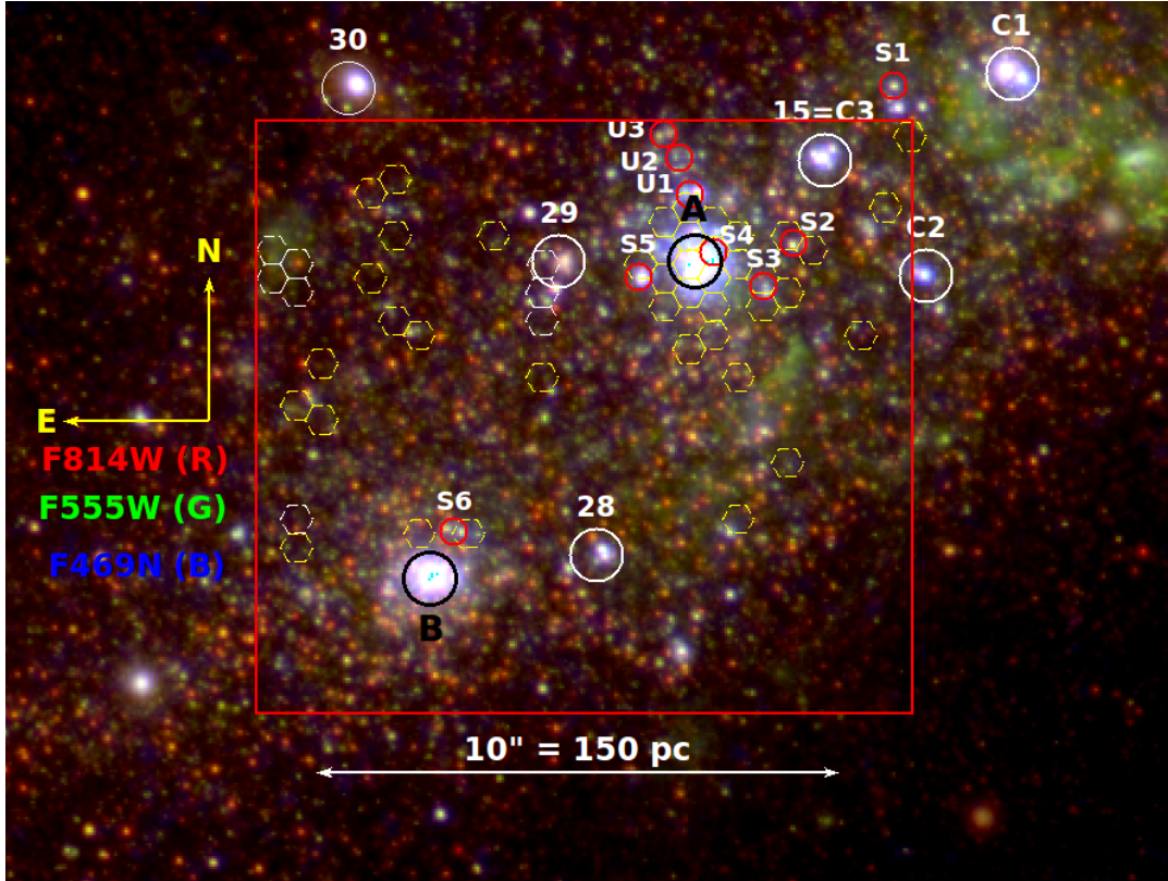
Figure 3. A colour-composite RGB image of the central starburst zone of NGC 1569. The image is formed by combining HST F814W, F555W and F469N band images, as red, green and blue components, respectively. MEGARA/IFU FoV ( 12.5 \text{ arcsec} \times 11.3 \text{ arcsec} ; red rectangle) and image orientation (compass) are shown. The locations of the fibres where we detected a broad He II \lambda 4686 component are shown by hexagons. The prominent objects in the FoV are identified. These include the two massive clusters SSC-A and SSC-B, and four other clusters (15, 28, 29 and 30) from Hunter et al. (2000) . WR sources identified by Buckalew et al. (2000) using the displayed HST F469N image, which intercepts the He II \lambda 4686 line, are shown. These include four clusters with WR stars (C1, C2, C3 and C4) and six WR stars (S1, S2, S3, S4, S5 and S6). Three sources (U1, U2 and U3) classified as of unknown origin by Buckalew et al. (2000) are also shown. The He II \lambda 4686 broad feature is detected in 18 adjacent fibres associated to SSC-A. The circles enclosing cluster candidates have a diameter of 1 arcsec, and hexagons have an equivalent diameter of 0.62 arcsec.
