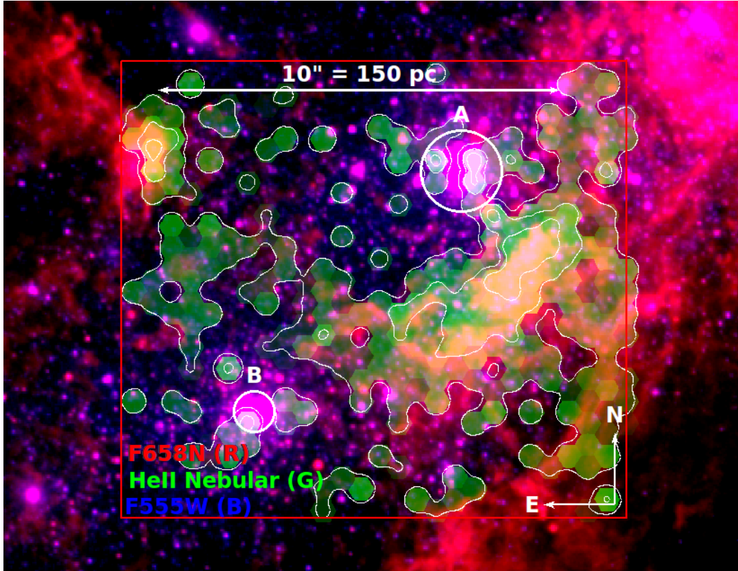
Figure 5. Colour-composite RGB image showing the morphology of the He II \lambda 4686 nebular emission (white contours englobing green hexagons) with respect to that of the H \alpha emission ( HST F658N-band shown in red) and stellar continuum ( HST F555W image shown in blue). Clusters A and B are marked. The contours corresponds to surface brightness levels of 3, 12 and 20 \times 10^{-17} \text{ erg cm}^{-2} \text{ s}^{-1} \text{ arcsec}^{-2} in the He II \lambda 4686 nebular line. The nebular emission is weak from SSCs A and B, and is distributed along a semi-circular arc with the most intense emission coming from a zone \sim 40 pc south-west of SSC-A.
