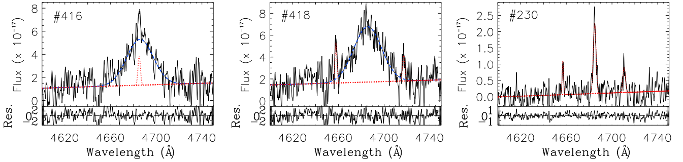
Figure 2. Multi-Gaussian fits to the blue bumps of individual fibres: broad He II \lambda 4686 line (blue), narrow He II \lambda 4686 nebular line (red) are shown for 3 representative fibre spectra that require: both the broad and narrow components (left; fibre#416), only the broad component (middle; fibre#418), and only the narrow component (right; fibre#230). The fitted continuum is shown by the red straight line, and the residuals of the fit are shown below each fit. The fluxes in the fitted spectra as well as in the residual are in units of 10^{-17} \text{erg cm}^{-2} \text{s}^{-1} \text{\AA}^{-1} . The middle and right spectra show additional narrow lines that we attribute to [Fe III] \lambda 4658 and He I \lambda 4713 nebular lines.
