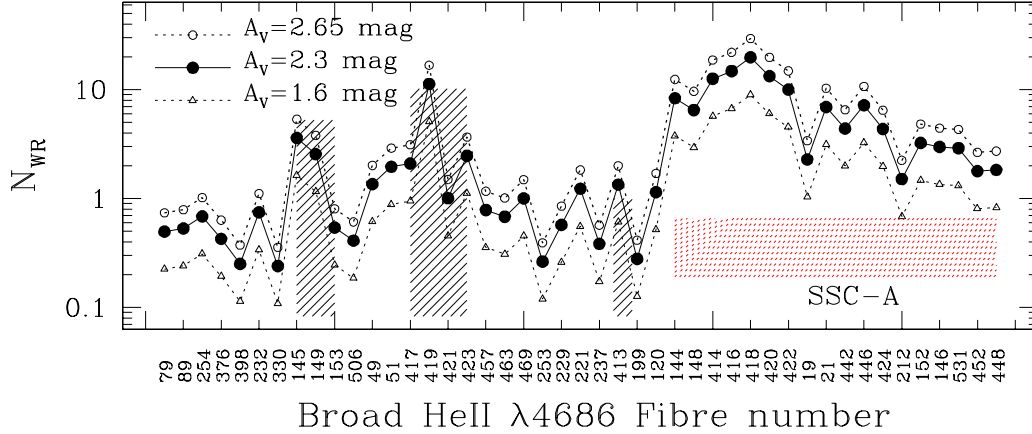
Figure 8. The number of WR stars, defined as the observed He II \lambda 4686 broad line luminosity divided by the typical luminosity of a WNL star ( 1.22 \times 10^{36} erg s ^{-1} ), vs fibre number. All 50 individual fibres where we detected broad He II \lambda 4686 feature are shown. The numbers are plotted for three values of extinction: A_V=1.6 mag, the minimum along the line of sight to NGC 1569 (triangles), A_V=2.65 mag, the mean determined for the ionized nebula (open circles), and A_V=2.3 mag, optimum value for SSC-A (solid circles). Fibres belonging to SSC-A, and those that have cross-talk with fibres of SSC-A are indicated by red shaded area, and diagonally hatched area, respectively. SSC-A contains 124 WR stars for A_V=2.3 mag.
