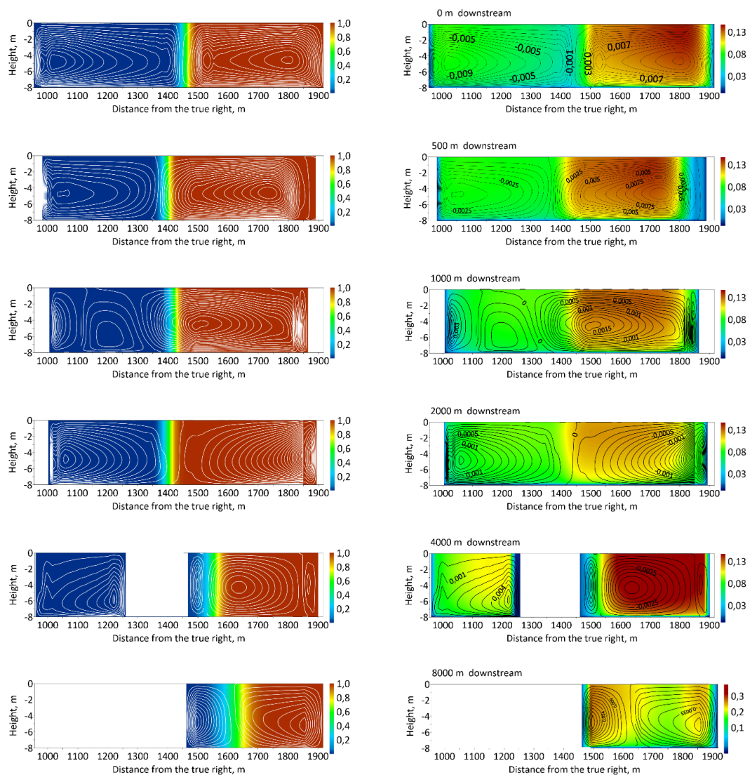
Figure 7. Predictions of concentration (left) and primary velocity (right, m \cdot s^{-1} ) with the stream function for Q_r = 0.62 and the P simulation geometry. Contours of flux are shown (units of m^2 \cdot s^{-1} ) as calculated by the stream function. Plots are viewed looking upstream, such that the Kama is on the left of each plot (i.e., the true right) and the Vishera on the right of each plot (i.e., true left). The contour values are only shown on the primary velocity plots.
