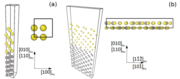
Fig. 1 Periodic simulation models used to compute the X/Fe ( X=\text{Au} or \text{Ag} ) interface energies, 3D and top views (shown here for X=\text{Au} ). (a) X(100)/\text{Fe}(100) ; (b) X(111)/\text{Fe}(110) . Fe atoms are depicted in gray, Au atoms in yellow. The axes refer to the top views.
