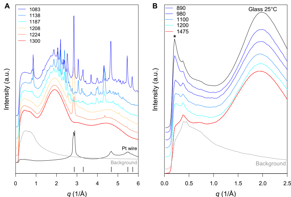
Fig. 2. In situ synchrotron XRD patterns of molten Mt. Etna basalt during slow and fast cooling. In (A), the Mt. Etna basalt was cooled at 1°C min -1 in air starting from pure melt at 1300°C down to 1083°C. Results show the microlite crystallization for 60-s acquisitions at the temperatures indicated. The sharp Bragg peaks at 1224° and 1208°C represent a “spinel-structured” phase. Plagioclase peaks appear from 1198°C. The sharp peak observed at 2.9 Å -1 in the melt at 1224°C is the 2 2 0 Bragg diffraction peak of crystalline Pt (black tick positions), arising from incident x-ray beam impinging on the Pt-Rh10% heating wire as it contracts. The spectra in (B) are for a much faster cooling of Mt. Etna basalt from 1475°C to room temperature (in black) and then to each target temperature in the legend, in a pure Ar atmosphere. The asterisk (*) indicates the small-angle “nanolite peak,” which increases systematically with deeper undercooling. Note the absence of Bragg peaks. All data are displaced vertically. The background curve shows the XRD measurement performed with an empty cell and results from the Kapton window enclosing the wire furnace.
