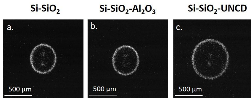
Figure 12 : Single shot ICCD image of plasma generated on the Si-SiO 2 bilayer (left) (a.), Si-SiO 2 -Al 2 O 3 trilayer (b.) and Si-SiO 2 -UNCD trilayer (c.) in the same operating conditions, at an applied voltages of 2 kV. The time delay is fixed at 21 ns and the exposure time is 4 ns.
