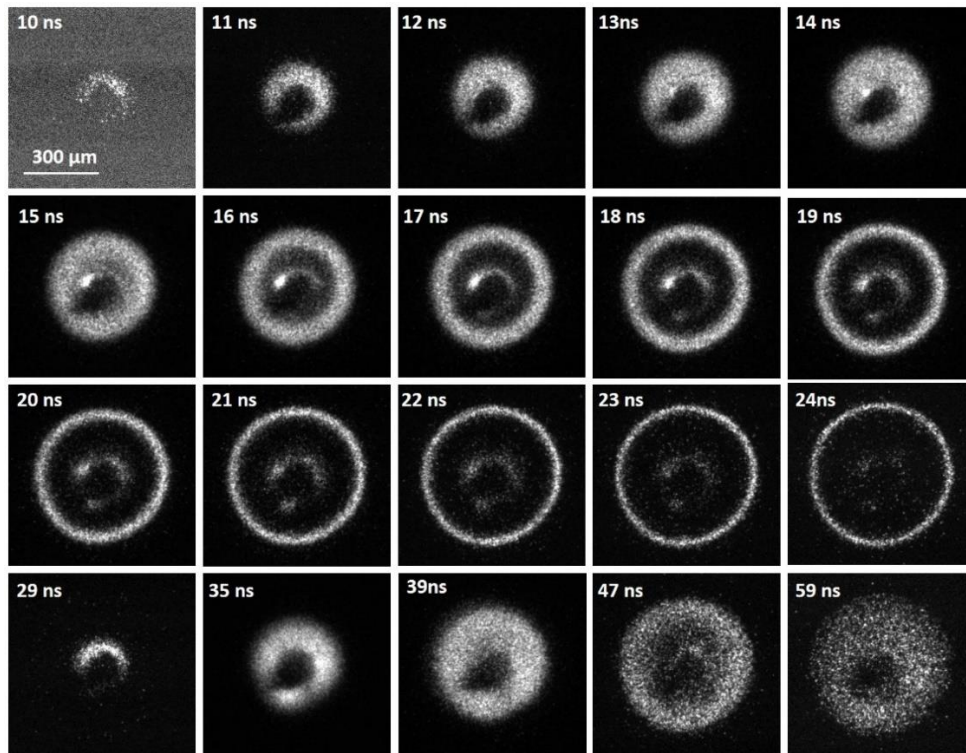
32 Figure 2 : Single-shot ICCD images of the plasma generated on the Si-SiO 2 bilayer, as a function of the delay 33 relative to the start of the voltage pulse at 0 ns. The applied voltage is 2 kV. The exposure time for each image is 34 4 ns.
