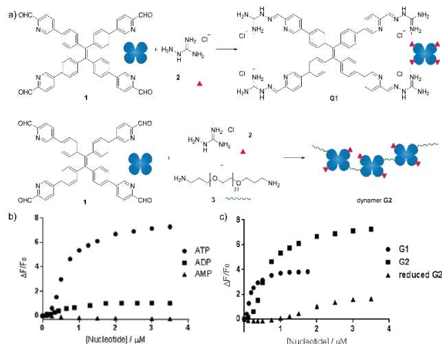
Figure 15. a) Syntheses of AIE based sensor G1 and dynamer G2 ; ATP sensing study by fluorescence spectroscopy of b) selective detection of ATP among other nucleotides by dynamer G2 ; c) ATP detection of dynamer G2 , compared to monomer G1 and imine reduced G2 , demonstrating the importance of multivalent and dynameric effects. 142 Copyright 2018 Wiley-VCH.
