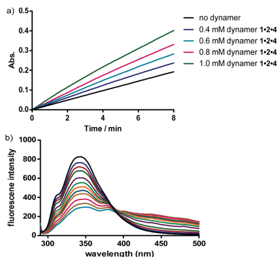
Figure 12. a) Representative UV time-course study of CA activity changes upon hydrolysis reaction of p-nitrophenyl acetate, showing increased activity by adding more dynamer 1-2-4 ; b) representative fluorescent titration study for CA-dynamer 1-2-4 interactions, the fluorescence intensity was gradually quenched with increasing amount of dynamer 1-2-4 . 137 Copyright 2016 The Royal Society of Chemistry.
