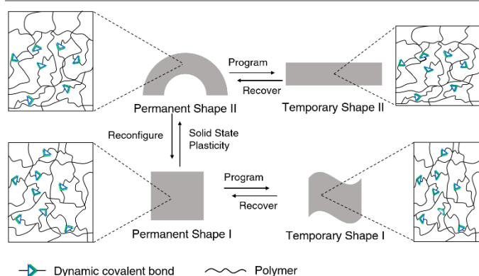
Figure 4. Reconfigurable shape memory dynamic covalent polymers.
