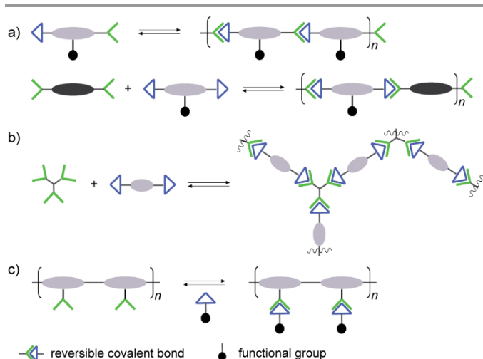
Figure 1. Different types of architectures in dynamic polymers with a) linear main-chain; b) cross-linked main-chain; c) side-chain connections. 19 Copyright 2017 American Chemical Society.
