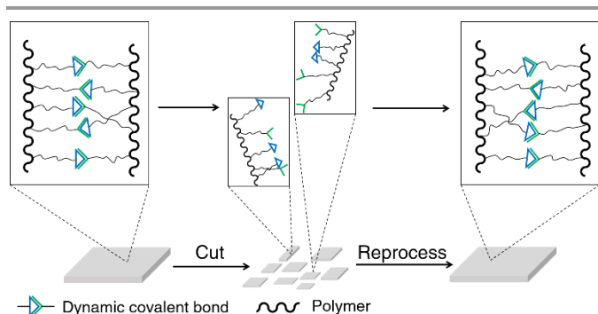
Figure 3. Illustration of the recyclability of dynamic covalent polymers.
