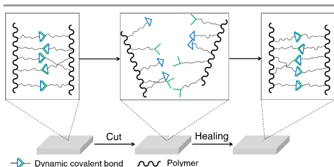
Figure 2. Illustration of self-healing dynamic covalent polymers.
