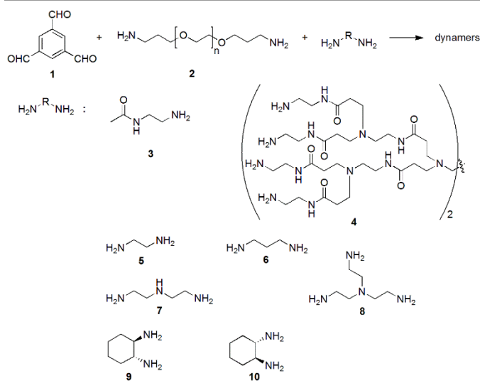
Figure 11. Syntheses of functional dynamic polymers for enzyme activation through imine formation reaction. 21, 139 Copyright 2016 The Royal Society of Chemistry.
