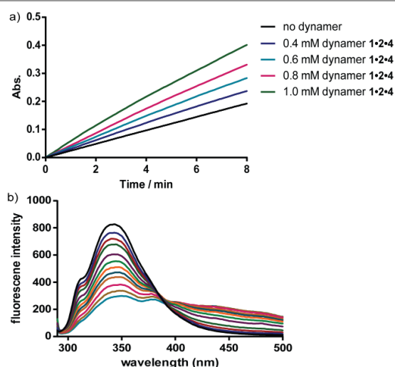
Figure 12. a) Representative UV time-course study of CA activity changes upon hydrolysis reaction of p-nitrophenyl acetate, showing increased activity by adding more dynamer 1-2-4 ; b) representative fluorescent titration study for CA-dynamer 1-2-4 interactions, the fluorescence intensity was gradually quenched with increasing amount of dynamer 1-2-4 . 137 Copyright 2016 The Royal Society of Chemistry.
