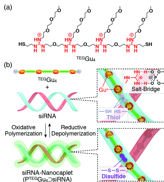
Figure 7. Nucleic acid-templated formation of redox-sensitive polydisulfide dynamic covalent polymers for siRNA delivery. (a) Molecular structure of water-soluble tetraguanidylated dithiol building block TEGGu 4 ; (b) principle of siRNA-templated oxidative polymerization and reductive depolymerization. Reproduced from ref. 113, 114 . Copyright 2015, American Chemical Society.
