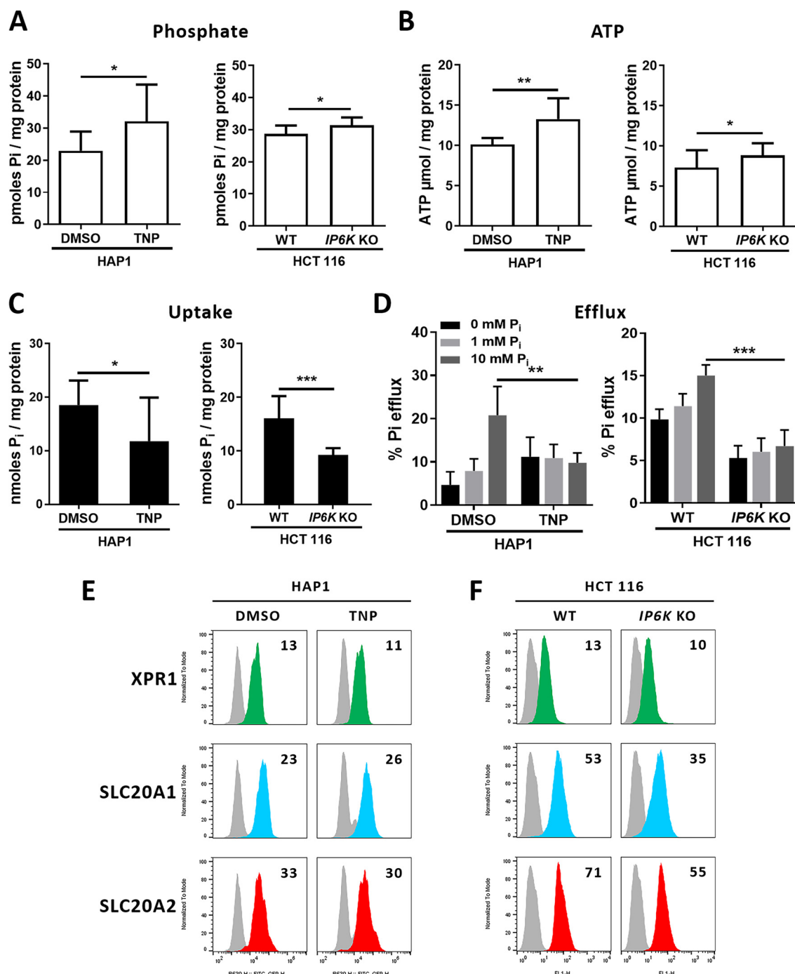
Figure 4. Inactivation of IP6K genes or kinase activity abolishes phosphate efflux regulation. A and B, levels of intracellular phosphate (A) and ATP (B) in HAP1 parental cells treated either with DMSO or with 10 \mu M TNP for 48 h and in parental or IP6K1-2 DKO HCT116 cells ( IP6K KO). Data are means \pm S.D. from 6 experiments. *, p \leq 0.05 ; **, p \leq 0.01 , two-tailed Student's t tests. C, uptake of [ ^{32} P]phosphate in HAP1 and HCT116 cells as in A. Data are means \pm S.D. from 3 experiments. *, p \leq 0.05 ; ***, p \leq 0.001 , two-tailed Student's t tests. D, efflux assays of [ ^{32} P]phosphate using the same cells as in A with efflux media containing different concentrations of phosphate. Data are shown as means \pm S.D. **, p \leq 0.01 ; ***, p \leq 0.001 , two-way ANOVA with Tukey's multiple-comparison test; left: F([P_i]) = 19.70 ( p < 0.0001 ); F(\text{cells}) = 0.2891 ( p = 0.5926 ); F(\text{interaction}) = 27.86 ( p < 0.0001 ); right: F([P_i]) = 385.7 ( p < 0.0001 ); F(\text{cells}) = 38.85 ( p < 0.0001 ); F(\text{interaction}) = 13.59 ( p < 0.0001 ); ***, p \leq 0.001 . E and F, cell surface detection of XPR1 (green), SLC20A1 (blue), and SLC20A2 (red) in HAP1 parental cells treated with either DMSO or TNP (E) and in HCT116 parental or IP6K1-2 DKO cells (F). Numbers indicate the specific change in mean fluorescence intensity of a representative experiment ( n = 3 ), compared with nonspecific staining with the secondary IgG (gray histograms). ns, nonsignificant; P_i , inorganic phosphate.
