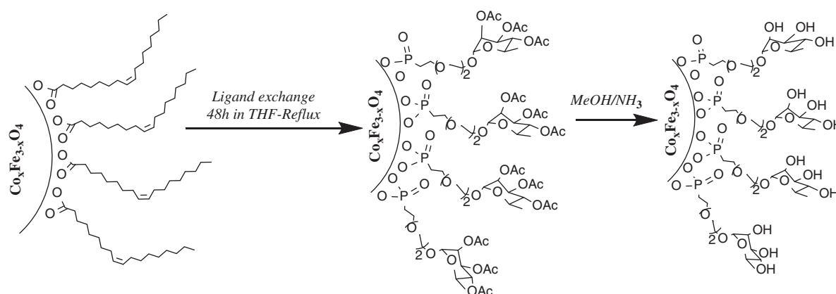
Figure 1. Schematic representation of the synthesis of rhamnose-functionalized \text{Co}_x\text{Fe}_{3-x}\text{O}_4 nanoparticles.
