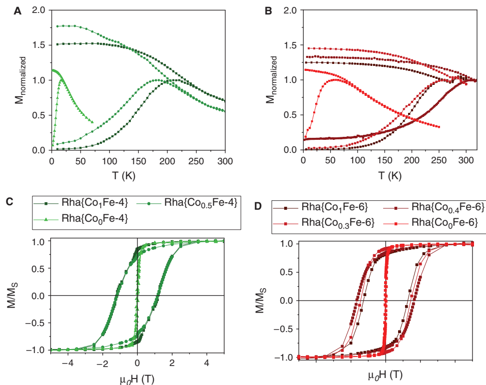
Figure 4. Experimental data from DC magnetic measurements of \text{Rha}\{\text{Co}_x\text{Fe}_{3-x}\text{O}_4\} nanoparticles. ZFC/FC curves performed in solution for series with mean diameter ca. 4 nm (A) and 6 nm (B). Hysteresis loops for the series of \text{Co}_x\text{Fe}_{3-x}\text{O}_4 nanoparticles of 4 nm (C) and 6 nm (D) performed in frozen solution at 2.5 K.
