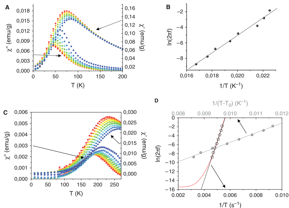
Figure 5. AC measurements for two samples of Rha { Co x Fe 3-x O 4 } nanoparticles. In phase, \chi' , and out-phase, \chi'' , components of AC susceptibility measurement for (A) Rha { Co 0 Fe-6 }, and (C) Rha { Co 1 Fe-4 } samples performed with 8 logarithmic spaced frequencies from 0.1 to 1000 kHz. Linear plot of \ln(2\pi f) versus 1/T_{\max} for (B) Rha { Co 0 Fe-6 } and (D) Rha { Co 1 Fe-4 } samples according to the Néel (dark), the Vogel-Fulcher (grey) and Torres et al. (red) model.
