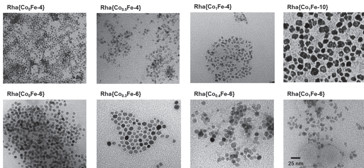
Figure 2. Representative TEM micrographs of \text{Co}_x\text{Fe}_{3-x}\text{O}_4 nanoparticles. The scale bar, reported in the last image, is the same over the series.
