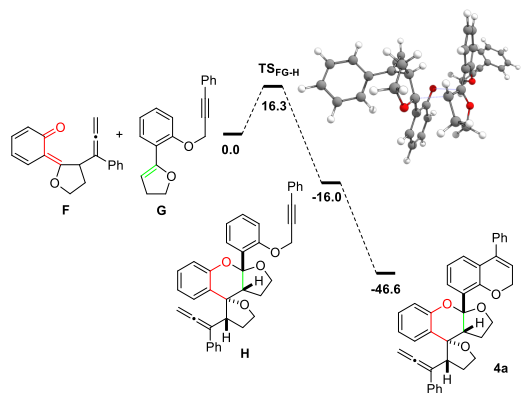
Scheme 5. Free Energy Profile ( \Delta G_{298} , kcal/mol) of the HAD, Geometry of TS_{FG-H} .
