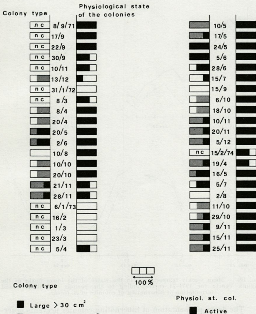
FIG. 9. — Pattern of change in the composition of population with time.
