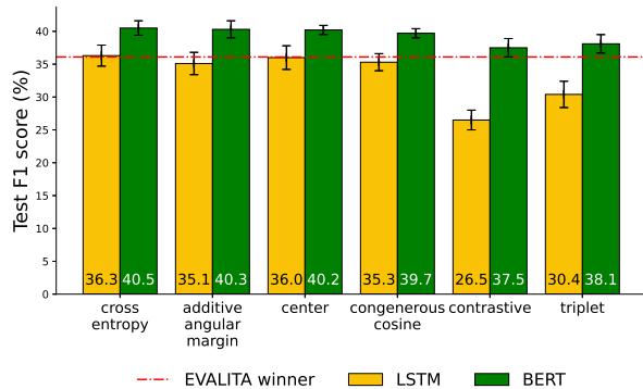
Figure 1: F1 scores on Test for each architecture and loss function. Scores are calculated as the mean of 10 runs and standard deviation is shown as error bars. The baseline of the Evalita 2018 winner (Ahluwalia et al., 2018) is shown for reference.
