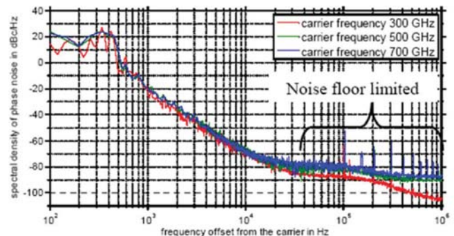
Fig. 2. Examples of the spectral density of the phase noise of the beat-note obtained when mixing the two frequencies from a DFL on a UTC photodiode (from IEMN). Note that the noise characteristics obtained without any control loop are almost the same when the frequency of beat-note is tuned from 300 to 700 GHz.
