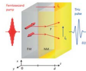
Fig. 7. Proposed original concept of THz emission based on spinorbitronics and spin-Hall effects in metallic multilayers. A fs laser pulse excites hot spin-polarized carriers at the interface between a ferromagnetic metal (FM) and a non-magnetic metal (NM). Spin relaxation generates ultrafast spin-currents and time-dependent charge oscillations.
