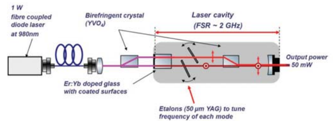
Fig. 1. Example of a solid state diode pumped dual frequency laser. The gain medium is a piece of Yb:Er co-doped glass, inserted within a cavity of 60 mm typical length. It delivers 10 mW output power on each optical frequency whose offset can be tuned, thanks to YAG etalons, over a typical 2 THz bandwidth. The “solid-state laser” approach provides both narrow linewidth, and low phase-noise on each optical component. The “single cavity” structure warrants a reduced phase noise of the beat-note, even without control loop.
