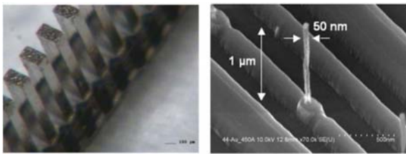
Fig. 4. Example of a THz slow wave structure realized using LIGA technique (20 to 200 \mu\text{m} typ. period with an aspect ratio > 1:10 ) (left). Example of a CNT grown on a "diffractive" structure. It provides an alignment of the polarization of the modulated optical beam (i.e. of the corresponding electric field) onto the main dimension of the CNTs (right).
