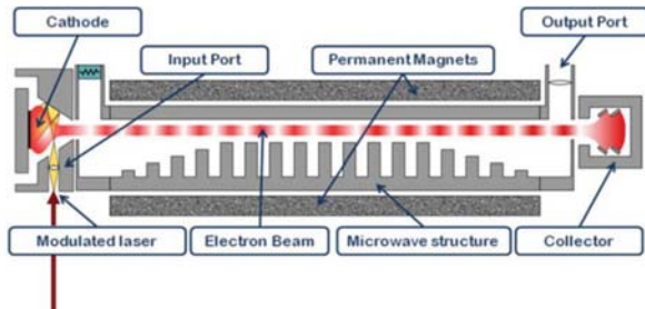
Fig. 3. Operating principle of an optically excited THz travelling wave tube. The cathode is made of an ensemble of carbon nanotubes (CNTs), optically excited through a plasmonic structure which align and concentrate optical field at the apex of CNTs. Field emission of CNTs (i.e. electrons bunches) is modulated by a modulated or dual frequency laser beam through Fowler-Nordheim like effect.
