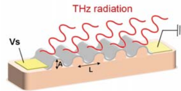
Fig. 6. Proposed original concept of a travelling wave THz source based on structured graphene. In phase synchrotron emissions from the periodically corrugated graphene layer is expected. Typical corrugations with A \sim 10\text{-}50 nm and L \sim 100\text{-}500 nm would result in an equivalent magnetic field of 100 T.
