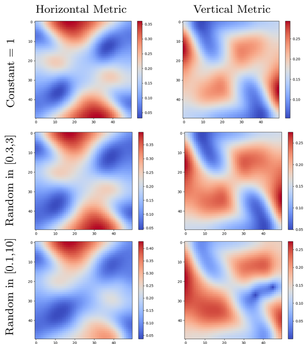
Fig. 10: We present the final metric of the experiment in Figure 4 for 3 different initializations: constant with weights equal to 1, random in log space in [0.3,3] , and random in log space in [0.1,10] . The algorithm is robust to a half order of magnitude in the metric weights, but not to a full one.
