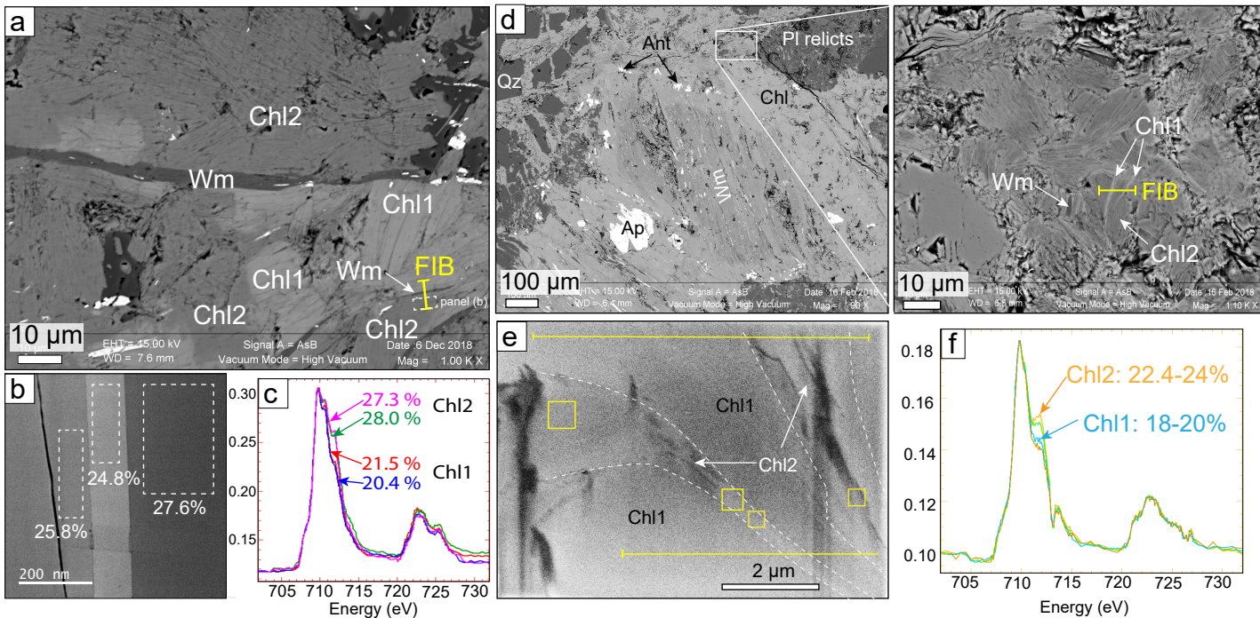
Figure S3 BSE, TEM images and XFe^{3+} estimates for mylonite ZA16-133 and little deformed sample ZA16-79. (a) Location of FIB section in a BSE image of sample ZA16-133. (b) TEM view of alternating chlorite crystallites in ZA16-133 with XFe^{3+} estimates. (c) Iron raw spectra for Chl1 and Chl2 along the FIB section and corresponding XFe^{3+} estimates. (d) BSE image of the location of FIB section in sample ZA16-79. (e) TEM view of the FIB section. Yellow squares: frames for EELS analyses at TEM. Yellow lines: profiles analysed by EELS and STXM. (f) Raw iron spectra for Chl1 and Chl2 along profiles and XFe^{3+} estimates for Chl1 and Chl2.
