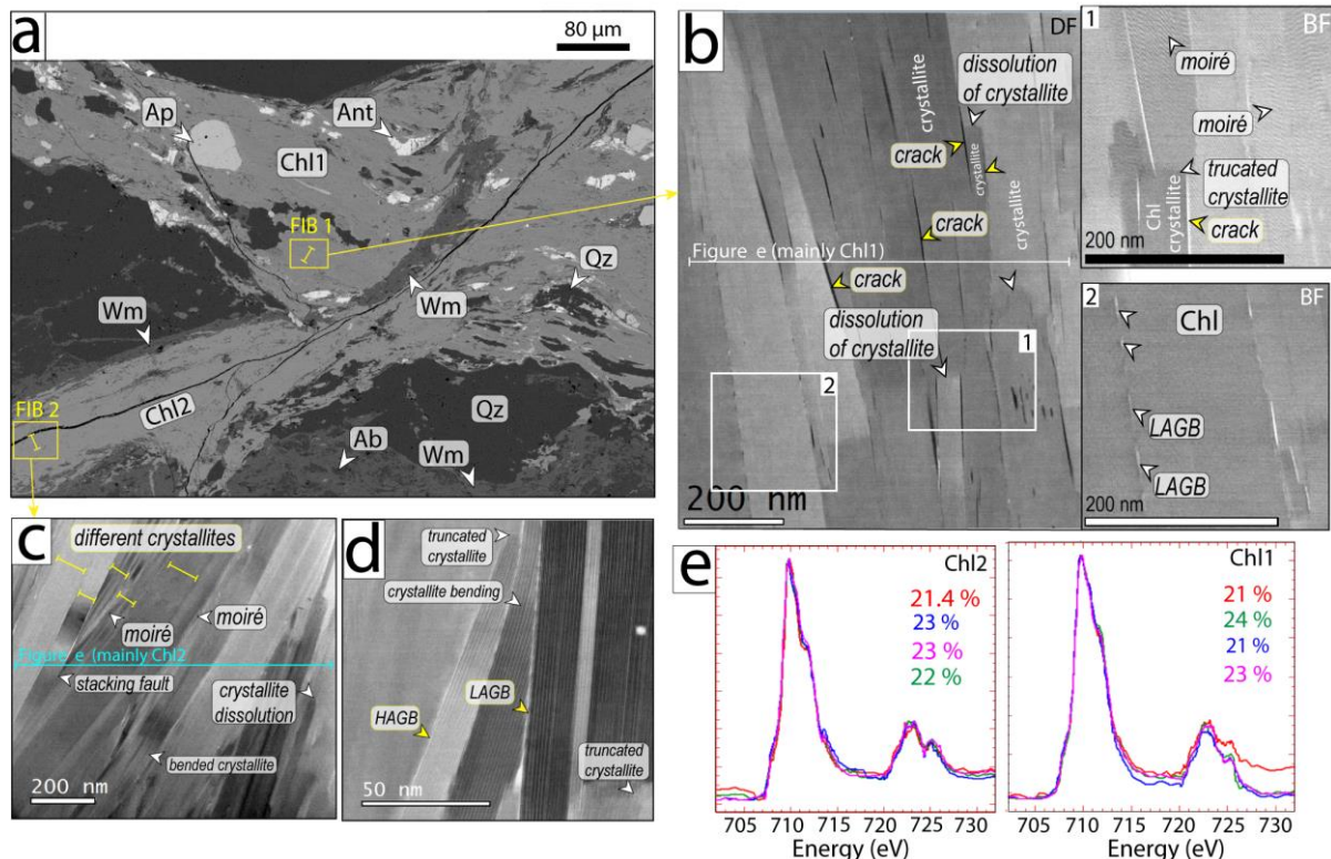
Figure 11 BSE, STEM images and XFe^{3+} (%) estimates in chlorite of mylonites (sample B10-31). (a) Location of the two FIB foils (in chlorite flakes where mainly Chl1 is observed and around crack where mainly Chl2 is observed) in BSE image corresponding to the composition map of Figure 6i. (b) STEM image of chlorite flakes in FIB section. (c) and (d) STEM images of chlorite around cracks (mainly Chl2) in FIB foil. (e) Raw iron spectra for Chl1 and Chl2-rich transects. The variation of XFe^{3+} (%) along a single transect in each chlorite is reported with coloured numbers (corresponding to different coloured spectra). DF: dark field, BF: bright field.
