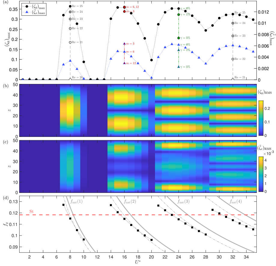
FIGURE 3. Responses of the flexible cylinder ( L/D = 50 ) at \text{Re} = 25 , for m = 6 and \gamma = 0 , as functions of U^* : (a) maximum amplitudes of displacement fluctuations in the CF (left axis; black circles) and IL (right axis; blue triangles) directions; (b,c) RMS values of the (b) CF and (c) IL displacement fluctuations along the span; (d) CF vibration frequency (IL vibration frequency is equal to twice this frequency). In (a), the maximum amplitudes of CF displacement for \text{Re} \in [20, 24] are also represented at U^* = 8 and U^* = 32 (grayscale circles); the maximum amplitudes of CF and IL displacement fluctuations are added for \text{Re} = 25 , at U^* = 16 for m \in \{3, 12\} and \gamma = 0 (red symbols), and at U^* = 24 for m = 6 and \gamma \in \{0.01, 0.05\} (green symbols). In (d), the natural frequencies of the first four structural modes in vacuum ( f_{\text{nat}} ) are indicated by plain gray lines; the corrected natural frequencies, with an added mass coefficient of 1, are denoted by gray dashed-dotted lines; the vortex shedding frequency identified by Buffoni (2003) is indicated by a red dashed line.
