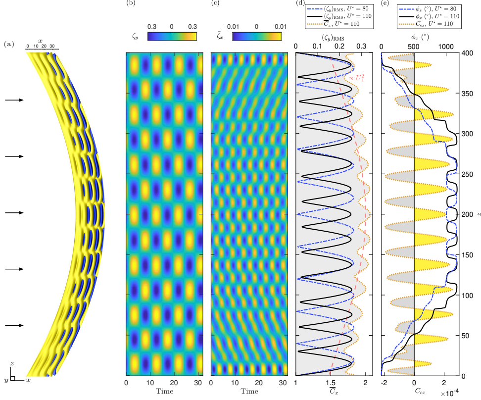
FIGURE 7. Flow-structure system behavior for L/D = 400 at Re = 25 : (a) instantaneous iso-surfaces of spanwise vorticity ( \omega_z \pm 0.07 ) for U^* = 110 (arrows represent the oncoming flow; part of the computational domain is visualized, i.e. 35D downstream of the cylinder); (b,c) time series of the (b) CF and (c) IL displacement fluctuations along the span for U^* = 110 ; (d) spanwise evolution of the RMS value of the CF displacement for U^* = 80 and U^* = 110 (top axis) and time-averaged IL force coefficient for U^* = 110 (bottom axis; gray area); (e) spanwise evolution of the local phase of the IL response ( \phi_x ) for U^* = 80 and U^* = 110 (top axis) and time-averaged power coefficient ( C_{ex} ) for U^* = 110 (bottom axis; regions of excitation/damping of the structure by the flow are represented by yellow/gray areas). In (d), a red dashed line indicates a possible trend of the mean force due to the cylinder streamwise deflection.
