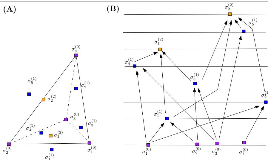
Figure 11 poly1(Eq. (19)): overview of critical points and Morse-Smale diagram
