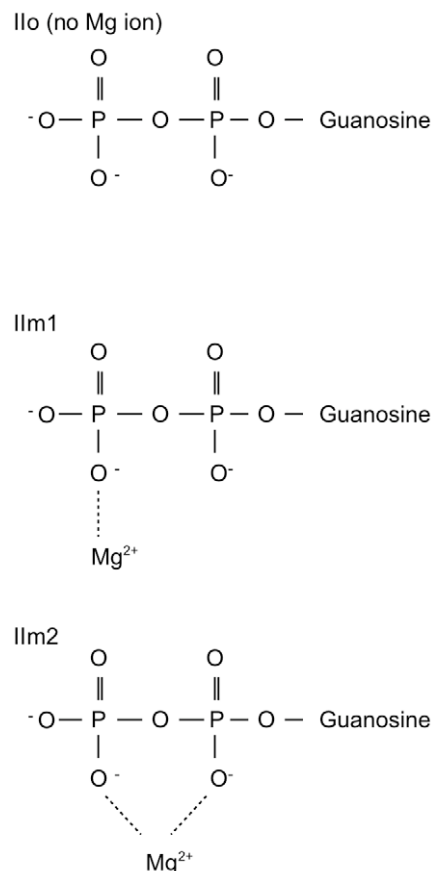
Figure 1. Mg 2+ placement for the three starting models of the Arf1-GDP-GEF complex.
