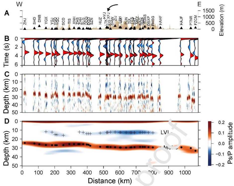
Figure 5 | Receiver function images of section P1. From top to bottom panels: A. Topographic profile, with triangles indicating station locations. The black arrow indicates the location of a giant quartz reef. B. Single-station stacked radial receiver function traces. Red pulses correspond to positive velocity gradients; blue pulses correspond to negative velocity gradients with depth. C. Individual receiver function traces plotted along profile representing raypaths of individual phase arrivals. D. Common conversion point migrated image with amplitudes indicated by color bar at right. Black dots represent the estimated Moho depth and crosses indicate the inferred top interfaces of the LVLs.
