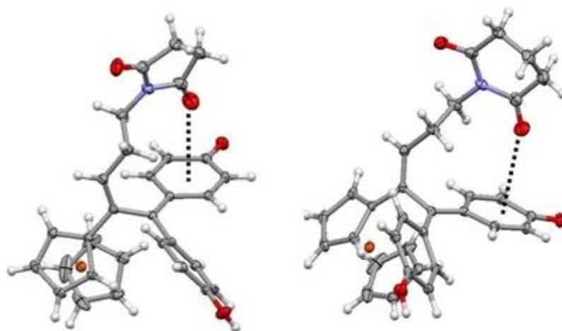
Figure 6. Molecular structures of (left) the succinimidopropyl-ferrocenyl-quinone methide 25 , with a stabilized lone pair- \pi interaction, and (right) the glutarimido analogue, 26 .
