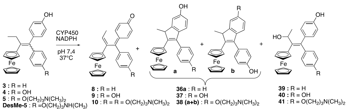
Scheme 10. Formation of the three main metabolites from phenols 3-5 . DesMe-5 is an additional metabolite of 5 .
