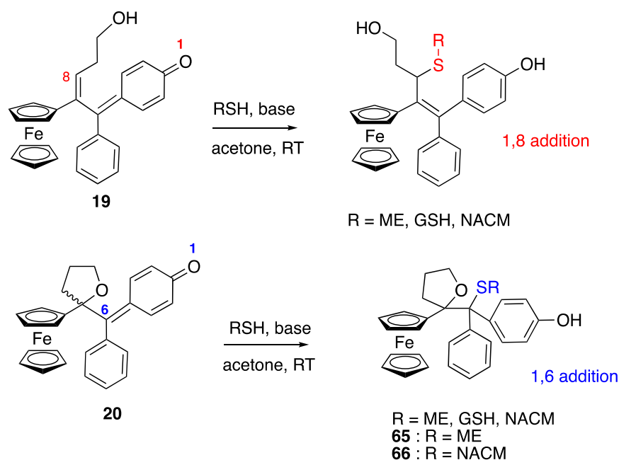
Scheme 16. 1,6- and 1,8-Michael additions of thiols to ferrocifenyl quinone methides.
