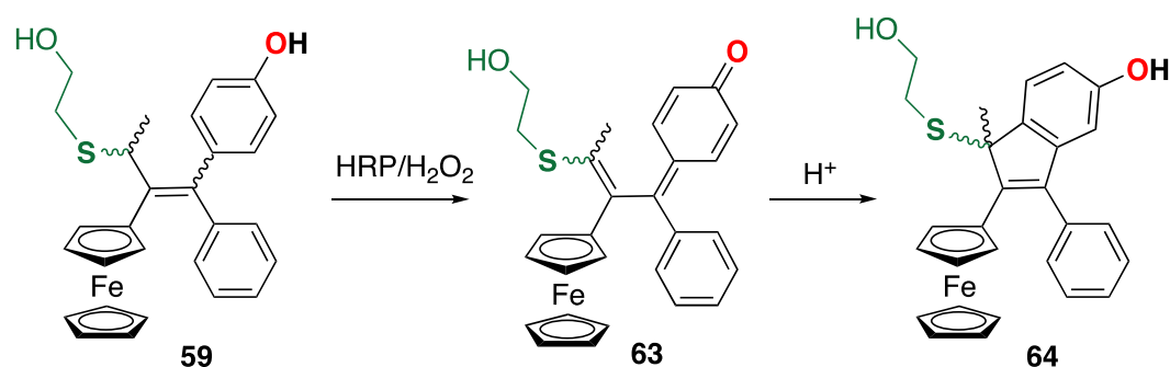
Scheme 15. Enzymatic oxidation of a ferrocifen-QM—thiol adduct, ultimately forming an indene.
