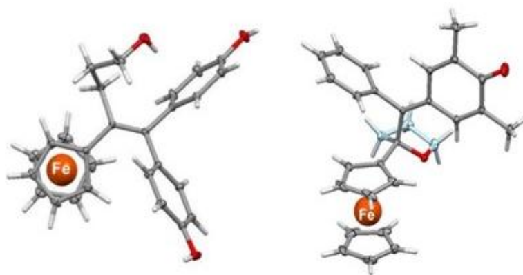
Figure 4. Molecular structures of (left) the hydroxypropyl-ferrociphenol, 17 , and (right) the THF-containing ferrocenyl quinone methide, 21 .
