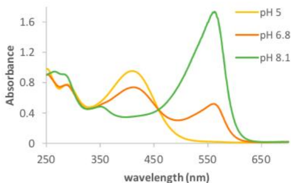
Figure 7. UV-Vis spectrum of ferrocidiphenol 4 after 2 min of incubation with HRP/H 2 O 2 at different pH values: phenolate 33 , 553 nm at pH 8.1; neutral phenol 9 , 406 nm at pH 5.
