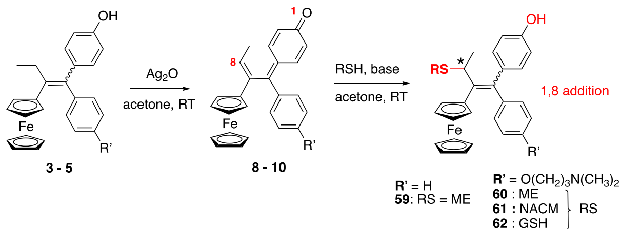
Scheme 14. 1,8-Michael additions of thiols, mercaptoethanol (ME), glutathione (GSH), N -acetyl- L -cysteine methyl ester (NACM), to a vinyl-ferrocifenyl-QM.
