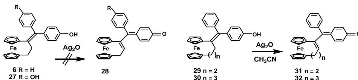
Scheme 7. Chemical oxidation of ansa-ferrociphenols yielded QMs only for n = 2 or 3 .
