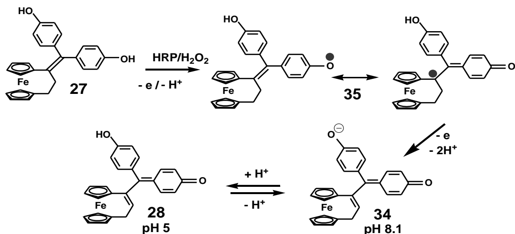
Scheme 9. Intermediacy of the short-lived, but detectable, ansa-QM radical 35 .
