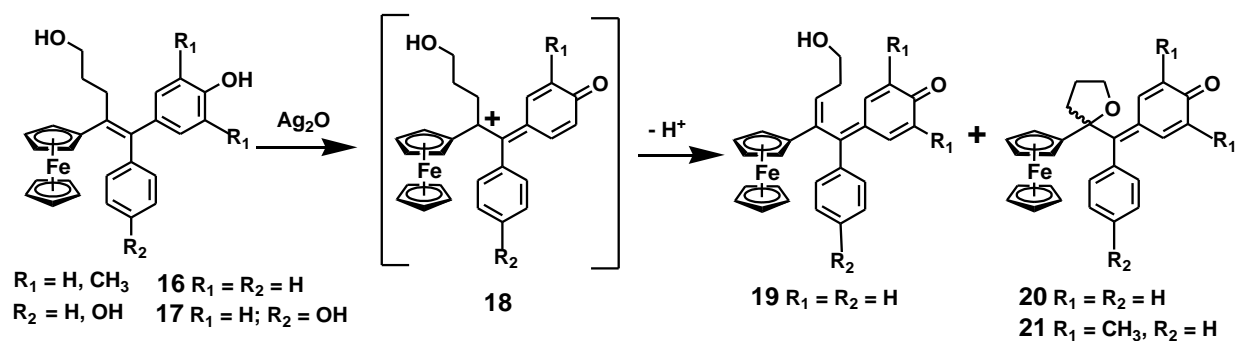
Scheme 4. Chemical oxidation of hydroxypropyl-ferrociphenols yields two different QMs.
