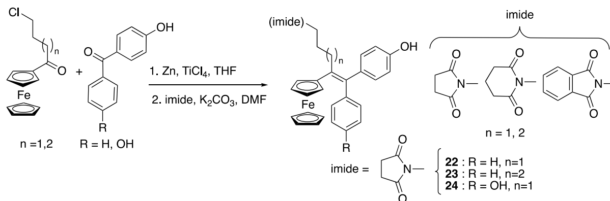
Scheme 5. Preparation of imidopropyl- and imidobutyl-ferrociphenols
