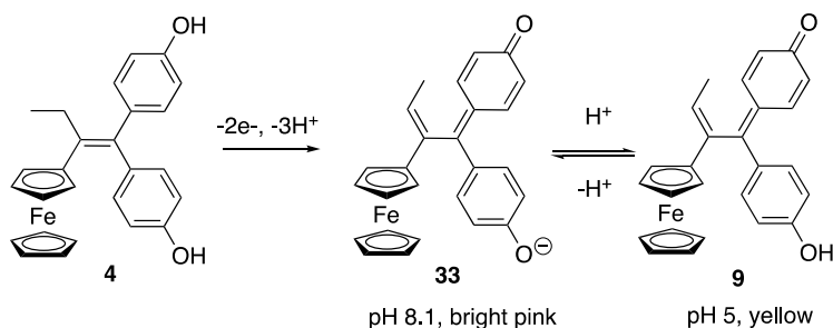
Scheme 8. Enzymatic oxidation of ferrocidiphenol 4 with HRP/H 2 O 2 yields, at pH 8.1, the QM in its phenolate form, 33 , and in its neutral form, 9 , at pH 5.
