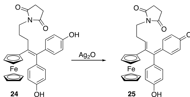
Scheme 6. Chemical oxidation of the succinimidopropyl-ferrocenyl-1,4-dihydroxybenzene 24 to form the succinimidopropyl-ferrocenyl-quinone methide 25 .
