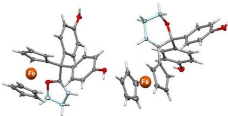
Figure 9. Molecular structures of (left) the dihydrofuran 56 and (right) the dihydropyran 58 .
