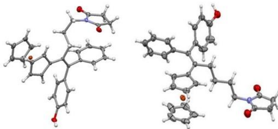
Scheme 5. Preparation of imidopropyl- and imidobutyl-ferrociphenols
