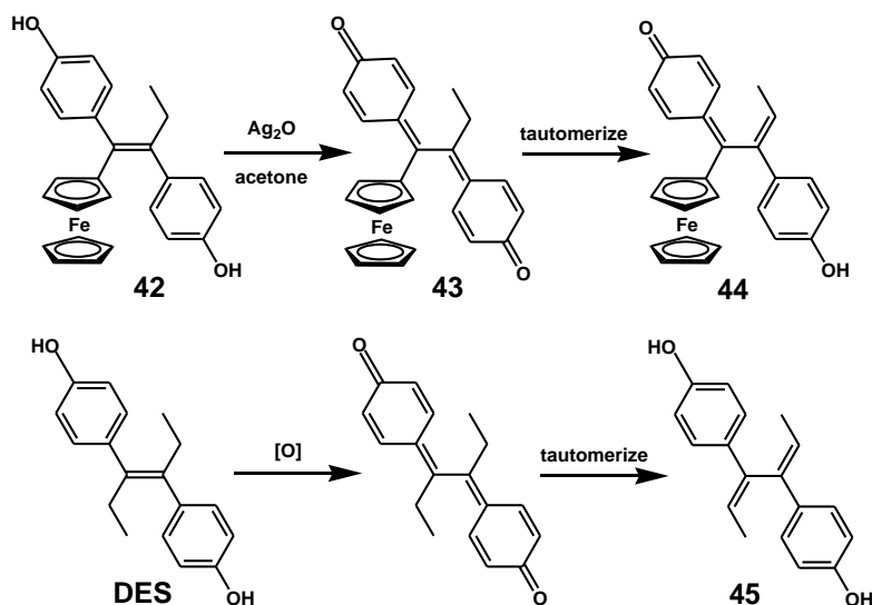
Scheme 11. Oxidation of ferrociphenol 42 , via diquinone 43 , to 44 .
