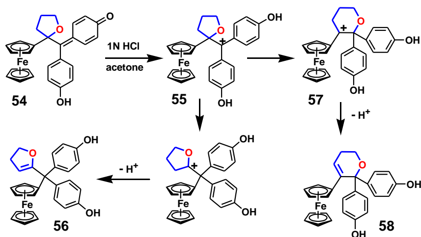
Scheme 13. Rearrangement of a protonated THF-quinone methide.
