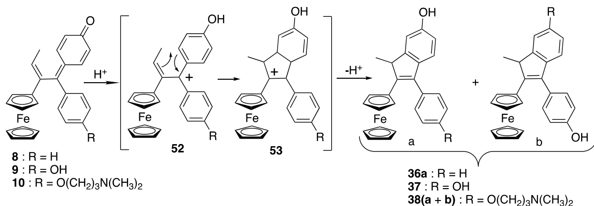
Scheme 12. Rearrangement of QMs into indenenes upon protonation.
