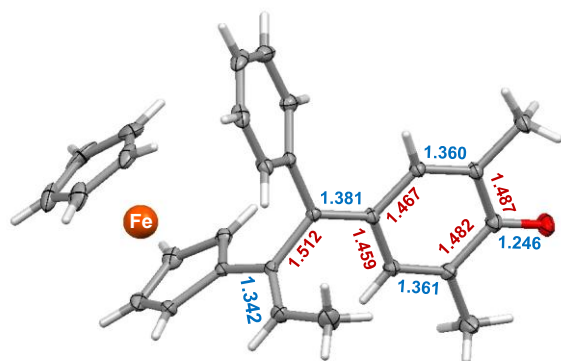
Figure 3. X-ray crystal structure of the ferrocenyl quinone methide E - 11 ; distances in Å.
