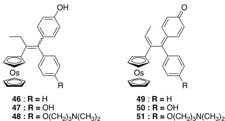
Figure 8. Osmocifens and their corresponding quinone methides.
