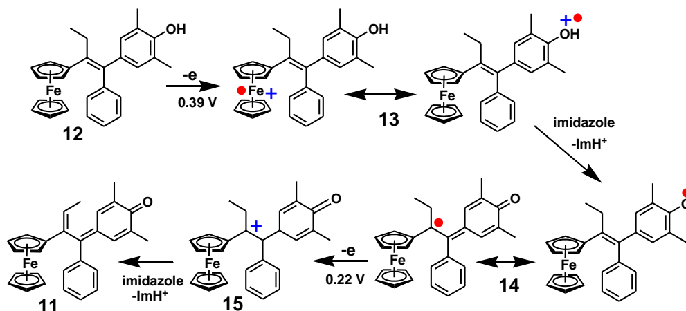
Scheme 3. Stepwise oxidation/deprotonation sequence to form a quinone methide.
