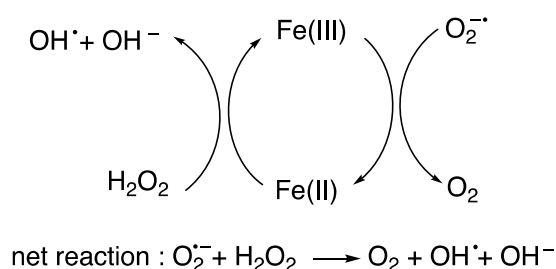
Scheme 17. The Fenton and Haber-Weiss reactions.
