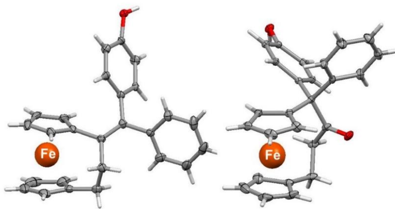
Figure 2. Molecular structures of (left) [3]ferrociphenol, 6 , and (right) its pinacolone rearrangement product, 7 .
