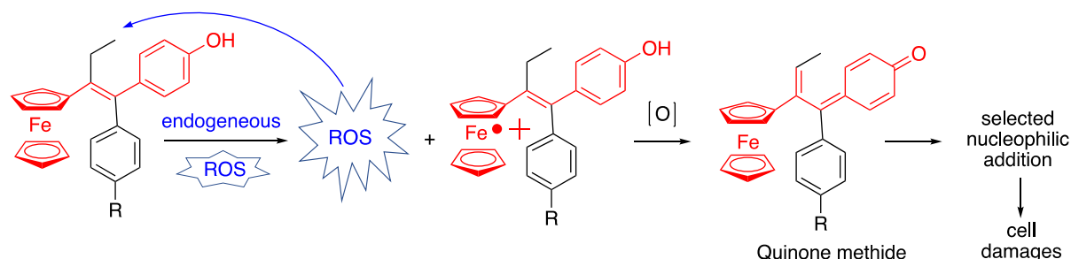
Scheme 18. Illustration of the kronatropic effect in cancer cells.
