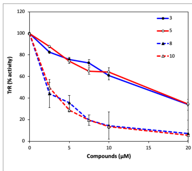
Figure 11. Thioredoxin reductase (TrxR1) inhibition by ferrociphenol 3 and hydroxyferrocifen 5 , and by their QMs 8 and 10 , respectively, when generated by chemical oxidation.
