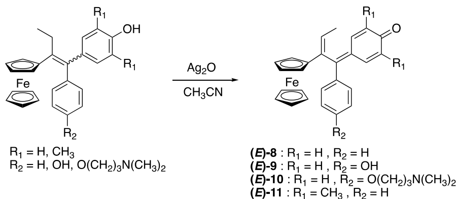
Scheme 2. Chemical oxidation of 3-5 leads to formation of quinone methides 8-11 .
