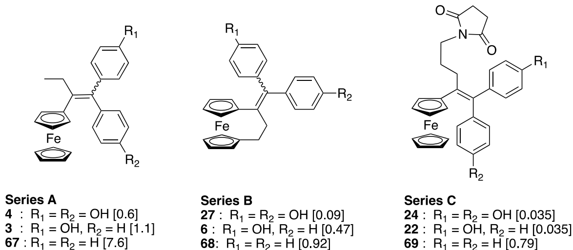
Scheme 19. Series of ferrocenyl complexes with zero, one or two OH groups. IC 50 values (μM) on MDA-MB-231 shown in square brackets are from Table S1.
