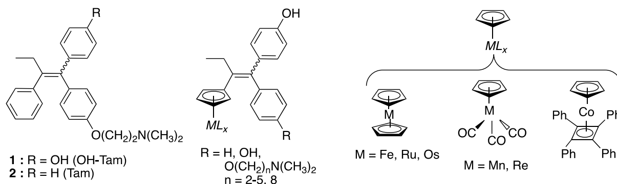
Figure 1. A selection of organometallic fragments incorporated into tamoxifen-type molecules.
