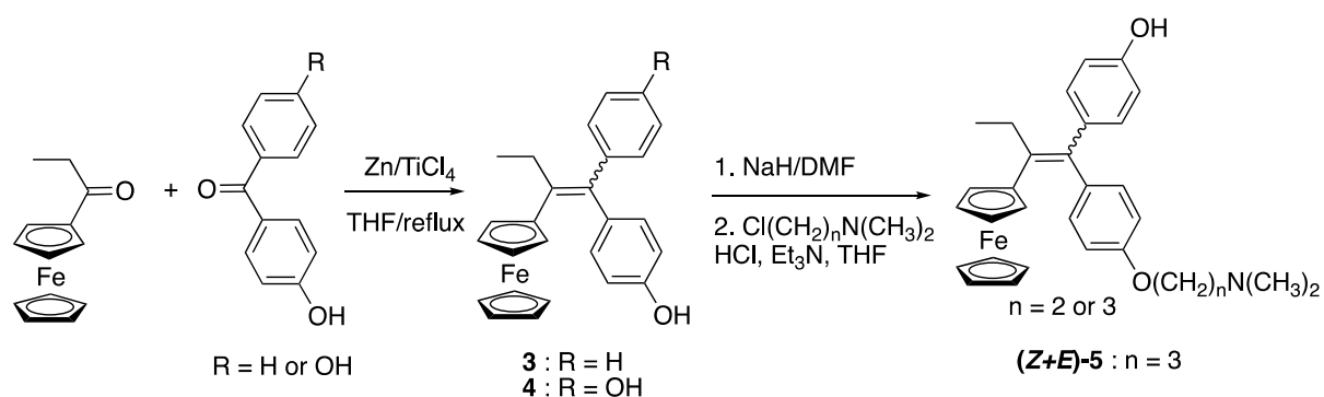
Scheme 1. Preparation of ferrociphenols and tamoxifen-like ferrocifens.
