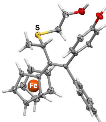
Figure 10. Molecular structure of the 1,8-mercaptoethanol adduct 59 .
