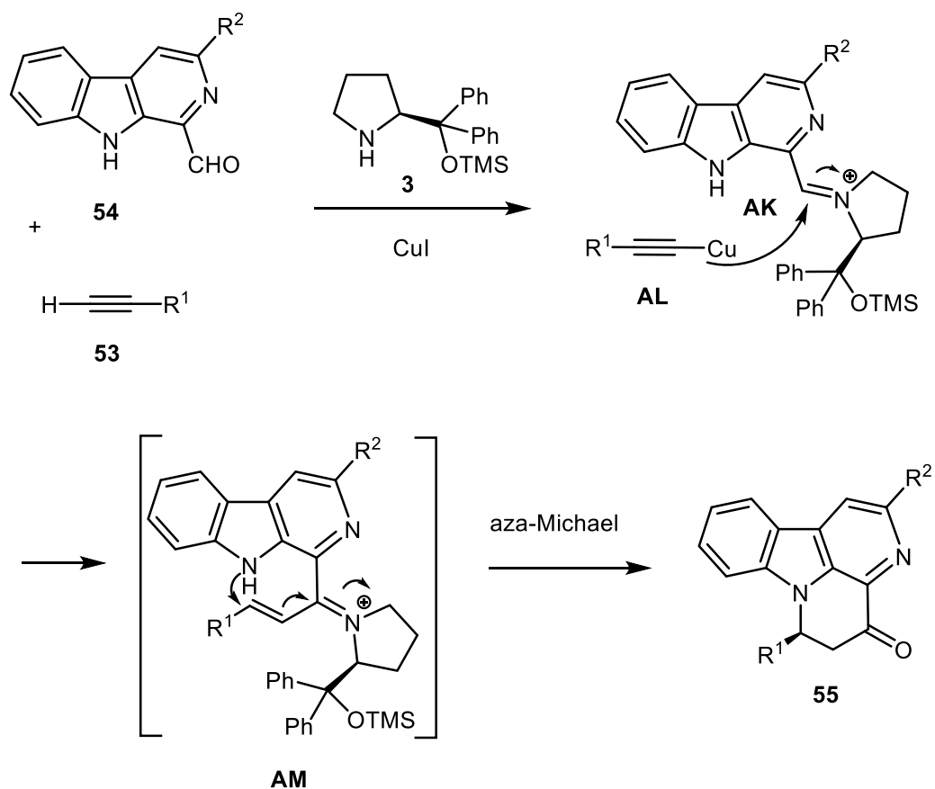
Scheme 17. Domino condensation/aza-Michael reaction of terminal alkynes with 1-formyl-9H-β-carbolines.
