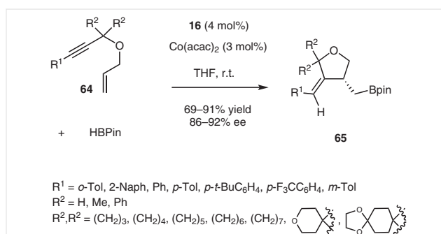
Scheme 17 Synthesis of other tetrahydrofurans through a Co-catalyzed domino reaction
