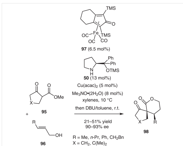
Scheme 25 Synthesis of bicyclic \delta -lactones through a multigated domino reaction
