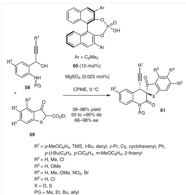
Scheme 15 Synthesis of spirocyclic dihydroquinolones through a Mg-catalyzed domino reaction
