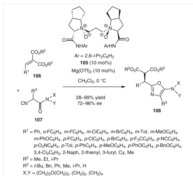
Scheme 27 Synthesis of 2-alkyl-5-aminoxazoles through a Mg-catalyzed domino reaction
