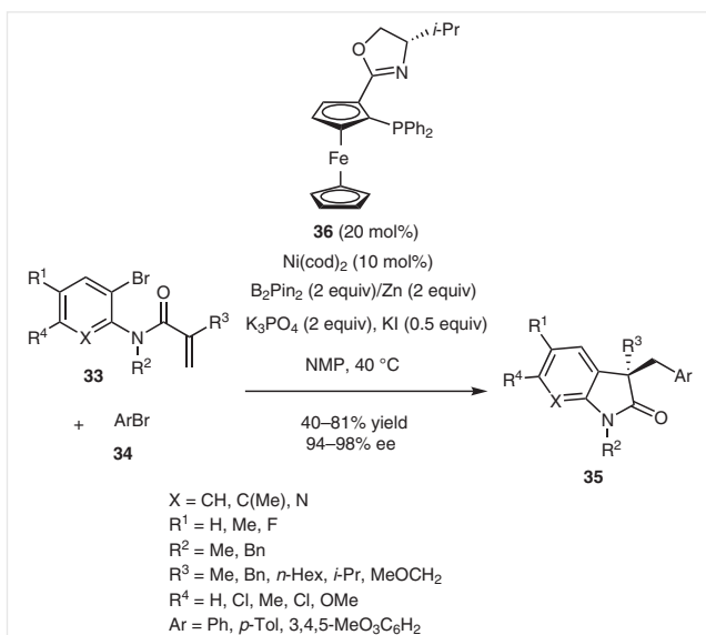
Scheme 9 Synthesis of bicyclic 2-pyrrolidinones through a Ni-catalyzed domino reaction
