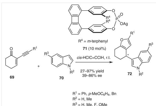
Scheme 19 Synthesis of bicyclic furans through an Ag-catalyzed domino reaction
