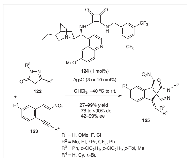
Scheme 32 Synthesis of spiroprazolones through a multicyclic domino reaction
