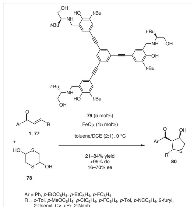
Scheme 21 Synthesis of tetrahydrothiophenes through an Fe-catalyzed domino reaction
