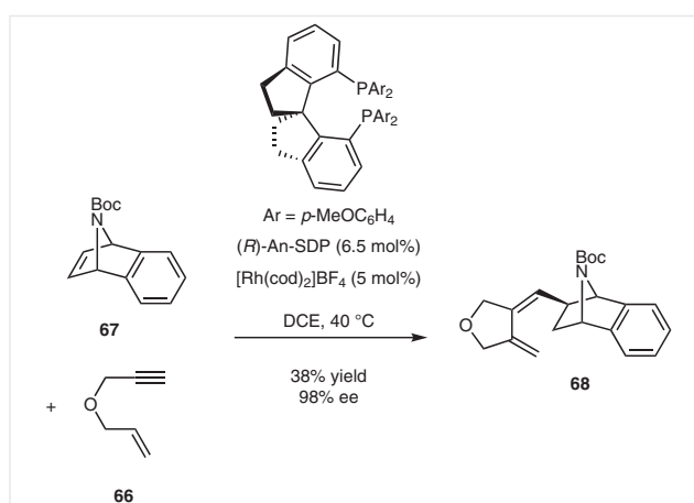
Scheme 18 Synthesis of a tetrahydrofuran through a Rh-catalyzed domino reaction
