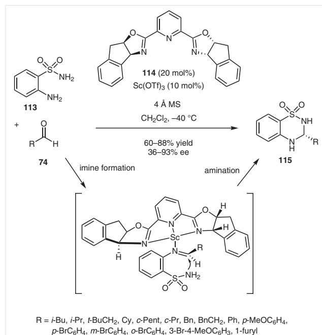
Scheme 30 Synthesis of 3,4-dihydro-2 H -1,2,4-benzothiadiazine-1,1-dioxides through a Sc-catalyzed domino reaction
