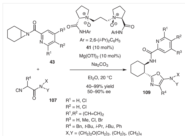
Scheme 28 Synthesis of other 2-alkyl-5-aminoxazoles through a Mg-catalyzed domino reaction
