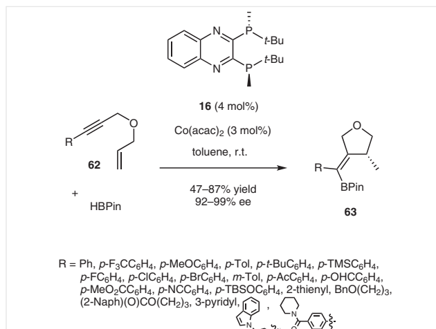
Scheme 16 Synthesis of tetrahydrofurans through a Co-catalyzed domino reaction
