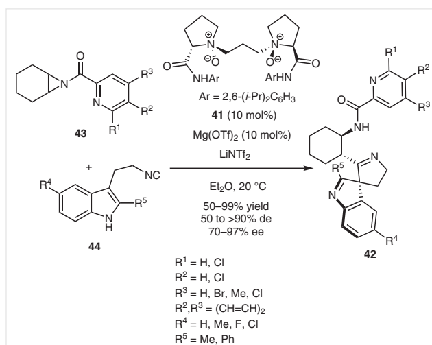
Scheme 11 Synthesis of spiroindolines through a Mg-catalyzed domino reaction
