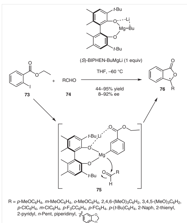
Scheme 20 Synthesis of 3-substituted isobenzofuranones through a Mg-catalyzed domino reaction
