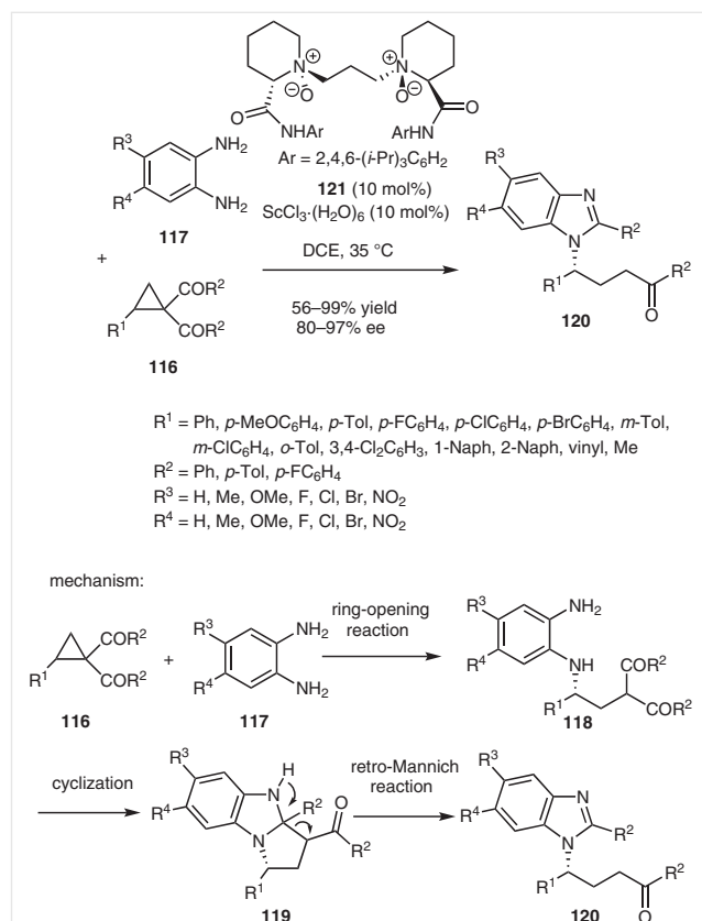
Scheme 31 Synthesis of benzimidazoles through a Sc-catalyzed domino reaction
