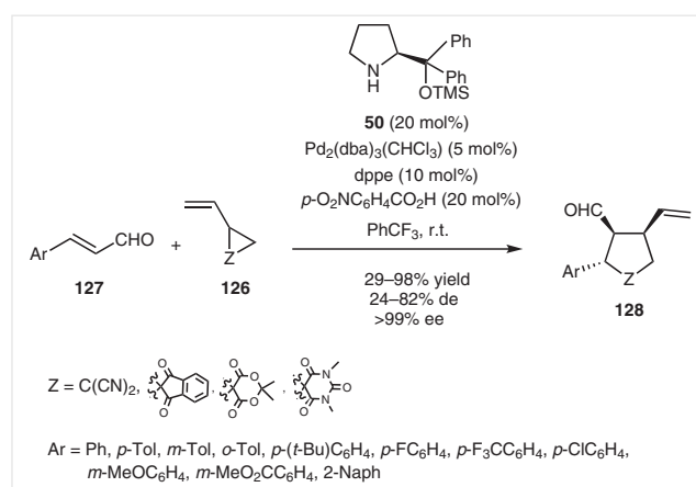
Scheme 33 Synthesis of trisubstituted cyclopentanes through a multicyclic domino reaction
