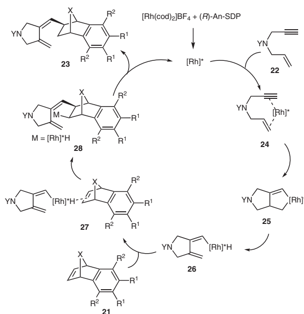
Scheme 7 Synthesis of 3,4-dimethylene-pyrrolidines through a Rh-catalyzed domino reaction
