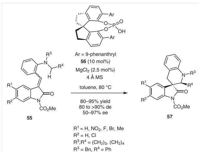
Scheme 14 Synthesis of spirooxindole tetrahydroquinolines through a Mg-catalyzed domino reaction
