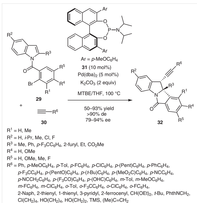
Scheme 8 Synthesis of 2,3-disubstituted indolines through a Pd-catalyzed domino reaction
