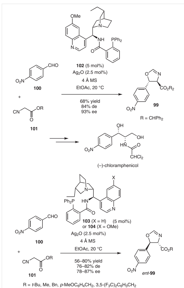
Scheme 26 Synthesis of oxazolines through Ag-catalyzed domino reactions
