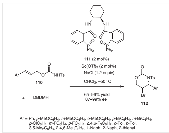
Scheme 29 Synthesis of aryl 5-bromo-1,3-oxazinan-2-ones through a Sc-catalyzed domino reaction
