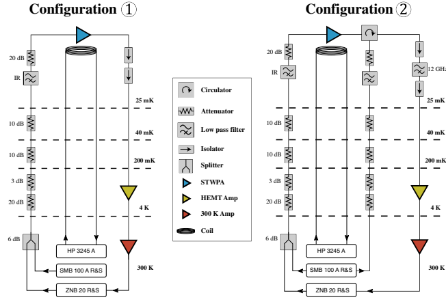
FIG. 12. Measurement setup. Configuration ① is a standard microwave transmission measurement setup. Configuration ② has one more input line. This configuration can be used for the same purpose as ① (pump and signal propagate in the same direction), or to probe backward gain (pump and signal propagate in opposite directions). Attenuators and filter of the leftmost and middle rf lines are nominally identical.
