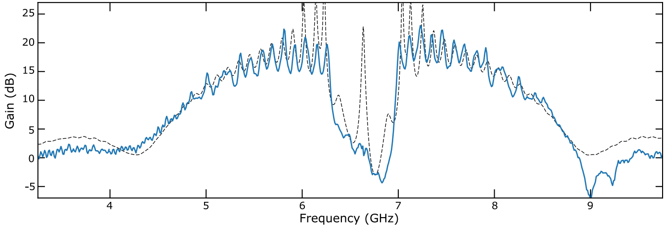
FIG. 3. Gain profile of the STWPA at magnetic flux \Phi/\Phi_0 = 0.2 and pump frequency 6.635 GHz and signal power P_s = -117 dBm. The theoretical gain profile (dashed black line) is obtained for a pump power P_{\text{input}} = -70.2 dBm.
