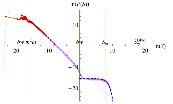
FIG. 13. Avalanche-size distribution P(S) for a particle with forces given by Eq. (6). The theoretical curves are the kicked ABBM model as given by Eq. (46) (cyan dotted), and the DPM as given by Eq. (62) (blue, dashed). INS, m^2 = 10^{-4} , \delta w = 1 , \delta t = 10^{-4} , S_m := \langle S^2 \rangle / (2 \langle S \rangle) = 2408.89 , \rho_m = 2329.95 , N = 10^8 .
