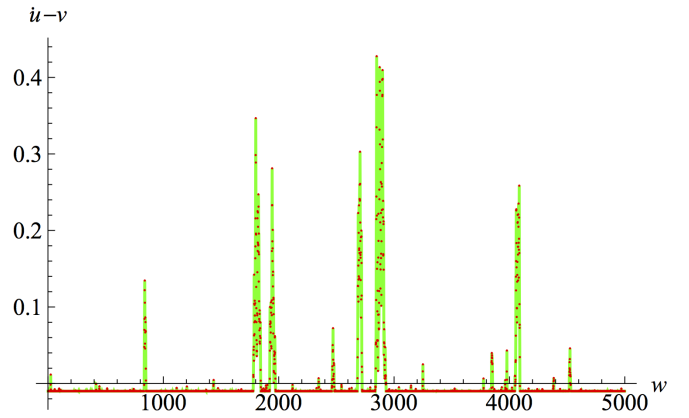
FIG. 4. \dot{u}_w - v with the same parameters as in Fig. 3.
