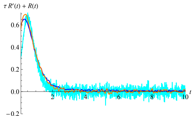
FIG. 10. The function \delta_{\text{BL}}(t) := (\tau \partial_t + 1)R(t) for the measured response function with m^2 = 10^{-2} (blue), m^2 = 10^{-3} (orange), m^2 = 10^{-4} (cyan). Parameters as in Fig. 9. ***plots missing, one could also put \delta_{\text{BL}}(t) on the y-axis.
