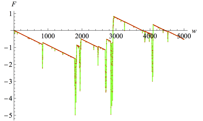
FIG. 5. F(w) with the same parameters as in Fig. 3.
