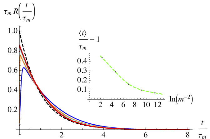
FIG. 9. The response function for the Ornstein-Uhlenbeck process: analytical result in black dashed. Numerical results from bottom to top are for m^2 = 10^{-2} (blue), m^2 = 10^{-3} (orange), m^2 = 10^{-4} (cyan), and m^2 = 10^{-5} (red). DNS, \delta t = 10^{-4} , N = 10^8 . The two larger masses have \delta w = 0.1 and \delta u = 10^{-6} , the two smaller ones \delta w = 1 , and \delta u = 10^{-4} . Inset: The measured timescale \langle t \rangle (dots) compared to the prediction for \tau_m in Eq. (64).
