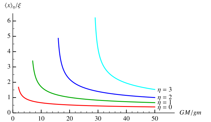
Figure 4. Mean distance \langle x \rangle_\eta / \xi of the impurity from the origin for the first four bound states as a function of GM/gm . At the threshold value for a given \eta , the mean distance diverges according to Eq. (55), signaling the disappearance of the bound state.
