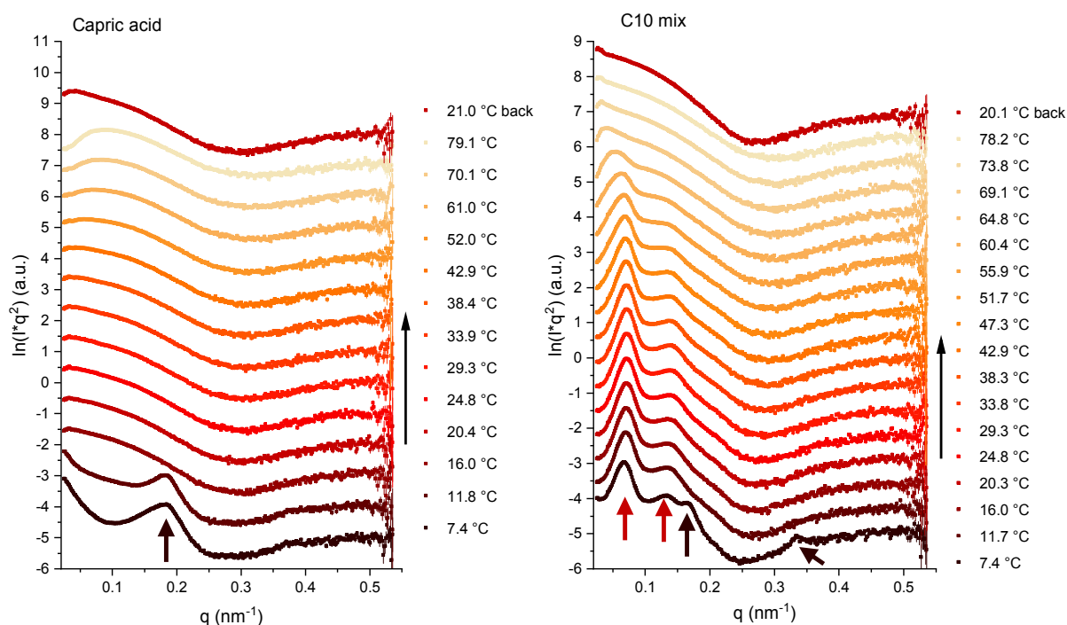
395 Figure 6. SANS curves at different temperatures collected on D16, shown in the representation \ln(I \cdot q^2) vs q , to highlight the presence of membrane correlations. This representation should flatten the curves that have the typical decay of vesicles ( q^{-2} ). Left: Capric acid sample 350 mM. Right: C10 mix sample 350 mM. Arrows show the first two orders of the observed lamellar phases structure factor S(q) .
