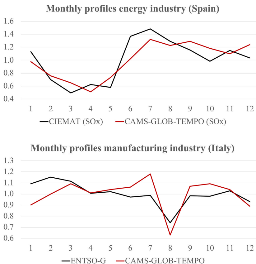
Figure 9: (Top panel) Comparison between monthly temporal factors for SO x energy industry emissions derived from power plant emission measurements (CIEMAT, personal communication) and reported by CAMS-GLOB-TEMPO for Spain. (Bottom panel) Comparison between monthly temporal factors for manufacturing industry emissions derived from real-world measurements of industrial natural gas consumption (ENTSO-G, 2020) and reported by CAMS-GLOB-TEMPO for Italy.
