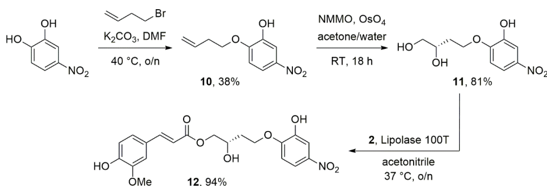
Scheme 1: Chemoenzymatic synthesis of (S)-4-O-(2-hydroxy-4-nitrophenyl)-1-O- trans -feruloyl-1,2,4-butanetriol (4NTC-linker-Fe, 12 ).
