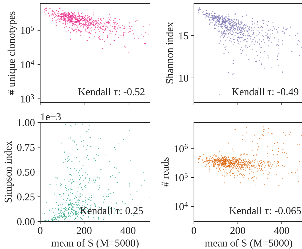
FIG. S2. Comparison between the mean of \mathcal{S} (autologous case), and three common diversity measures: the number of unique sequences found in the dataset (top left), the Shannon index, -\sum \hat{f}_s \ln \hat{f}_s (top right), the Simpson index (bottom left), and the total number of reads in each datasets (bottom right). All the diversity measures show a strong correlation with \mathcal{S} , but the correlation with the sequencing depth is low.
