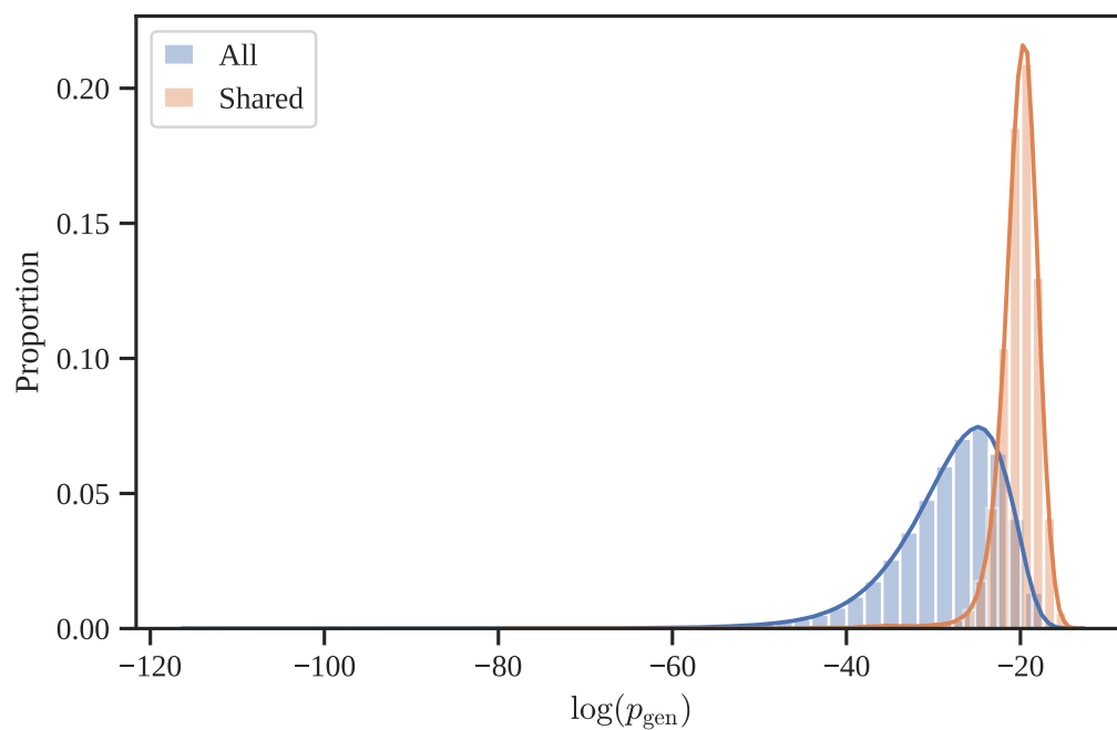
FIG. S11. Distribution of \ln(P_{gen}) for generic sequences, and for sequences shared between heterologous samples.
