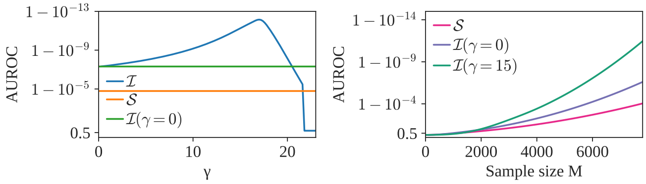
FIG. S8. Left panel: AUROC (Area Under Receiver Operating Characteristic) of \mathcal{I} , as a function of \gamma ( M = M_1 = M_2 = 5000 ). We observe an optimum near \gamma = 15 . Right panel: AUROC as a function of M , for \mathcal{S} , \mathcal{I}(\gamma = 0) , and \mathcal{I}(\gamma = 15) .
