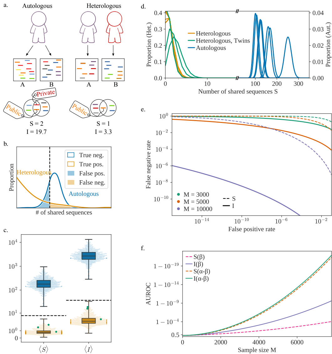
FIG. 1. a) The two samples A and B can either originate from the same individual (autologous) or two different individuals (heterologous). In both scenarios, sequences can be shared between the two samples, but their quantity and quality vary. b) Schematic representation of the distribution of the S or I scores for multiple pairs of samples extracted from the same individual (in the autologous scenario) or the same pair of individuals (heterologous). The dashed vertical line represents the threshold value. c) Expected value of S and I for different pairs of samples, sampled from the same individual (in blue) or different ones (yellow). Green dots represent samples extracted from pairs of identical twins. The dashed lines represent the theoretical upper bound for heterologous repertoires (see Methods) for both S and I ( \gamma = 12 ). d) Sampling distributions of S for 6 different patients (autologous case, each blue curve is one patient) or 6 different pairs of patients (heterologous, each yellow or green curve is a pair of patients) for M = 5000 . The y-axis scale on the left is adapted to the heterologous distributions while the scale on the right corresponds to the (much wider) autologous ones. The 3 sampling distributions in green correspond to a pair of samples extracted from identical twins. e) Detection Error Trade-off (DET) graph for both summary statistics and different sample sizes M . I ( \gamma = 12 ) outperforms S in all scenarios. f) AUROC (Area Under Receiver Operating Characteristic), as a function of M . The AUROC is a traditional measure of the quality of a binary classifier (a score closer to one indicates a better classifier). The results are shown for S and I both in the default case (only the \beta chain considered) or for the full ( \alpha - \beta ) receptor.
