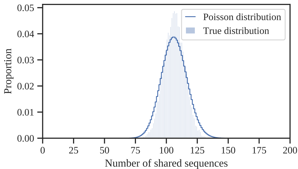
FIG. S10. Comparison between the distribution of \mathcal{S} obtained by computationally and repeatedly downsampling a single repertoire from Ref. [17] with M = 5,000 (histogram), and a Poisson distribution of the same mean (full line).
