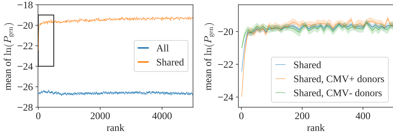
FIG. S7. Left: Mean value of P_{\text{gen}} as a function of the rank of the clonotype, for generic sequences (blue) and sequences shared between more than two donors (orange). The mean stays flat indicating that the probability of being generated does not generally depend on the clonotype size. There is an exception (black rectangle), shown as a close-up on the right panel. The top twenty clones, when shared between donors, have a smaller probability of being generated than expected by chance. This difference is likely to be driven by convergent selection against common pathogens, since CMV positive donors show a more pronounced effect than CMV negative ones.
