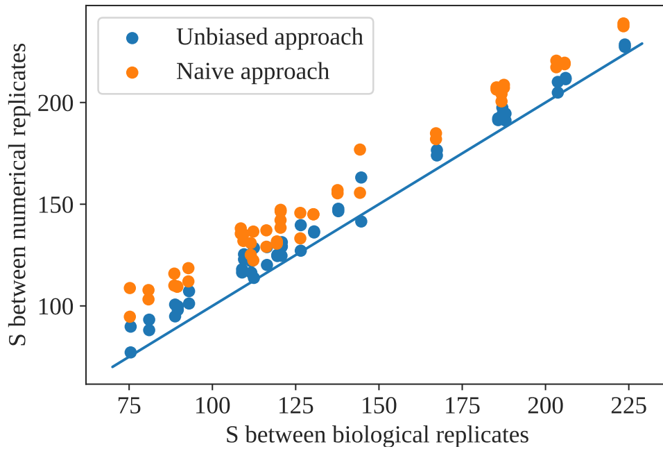
FIG. S9. Naive and corrected estimates of the autologous \mathcal{S} from single datasets, versus its values computed using true biological replicates from Ref. [18].
