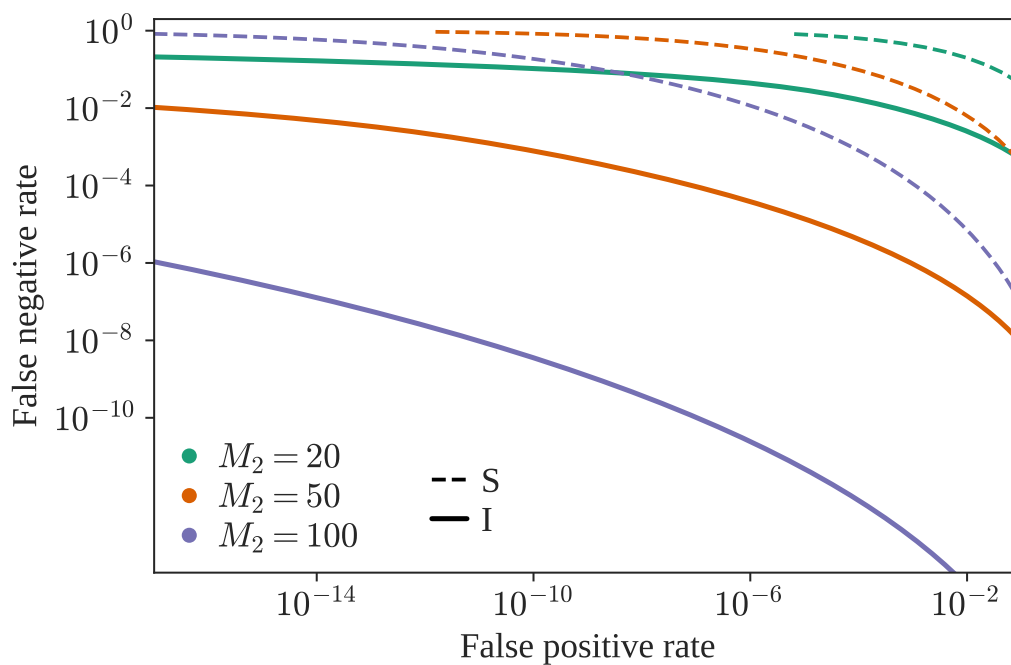
FIG. S3. Detection Error Trade-off (DET) graph for both summary statistics, between a large sample (full dataset, M_1 = 10^6 ) and a smaller one, of size M_2 = M .
