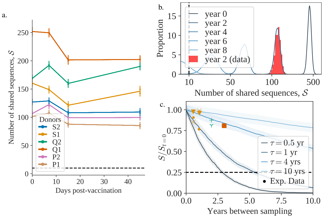
FIG. S5. a) Evolution of S ( M = 5000 ) during vaccination, between a sample taken at day 0 (vaccination date) and at a later timepoint. Each color represents a different individual. Each pair timepoint/individual has two biological replicates. The dashed line represents the threshold value. b) Evolution of S between a sample taken at year 0 and a later timepoint. The red histogram corresponds to one of the individuals sampled in [18] and the blue curves show theoretical estimates, fitted to match ( \tau = 0.66 ). c) Evolution of the (normalized) mean of S ( M = 5000 ) as a function of time for different values of the turnover rate \tau . The dashed line represents the threshold value divided by the smallest value of S_{t=0} ( M = 5000 ) in the data. The data points were obtained from the datasets [31] (yellow), [18] (green) and [22] (orange). Different markers indicate different individuals.
