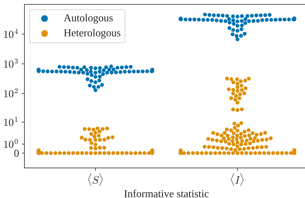
FIG. S4. Mean value of \mathcal{S} (left) and \mathcal{I} (right) for the IGH chain, part of the B-cell receptor, for sample sizes M = 5000 . The IGH sequences used are restricted to IgG+ B-cells (selected according to their CH gene). The sequences were obtained from 8 different individuals (6 biological replicates each) in the dataset from [30]. Autologous (blue) and heterologous (yellow) are well separated.
