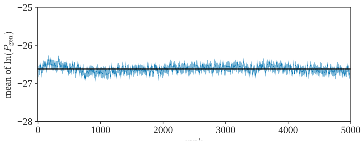
FIG. S1. Mean value of \log P_{\text{gen}} as a function of the rank of the clonotype (from most abundant to least abundant) from [17]. The black line represents the mean of \log P_{\text{gen}} for naive clones. The statistic for the top-clones (low rank) is similar to the one for the naive clones.
