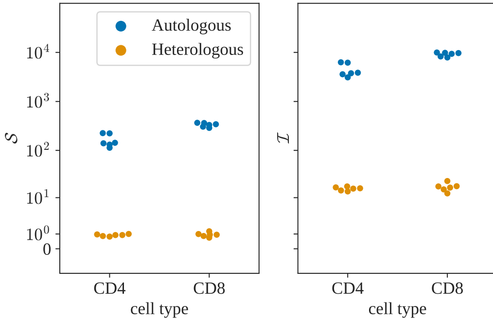
FIG. S6. Distribution of \mathcal{S} (left) and \mathcal{I} (right) for CD4+ and CD8+ T-cells in the dataset from [18] (6 individuals). In the autologous case (blue), there is a significant difference between the two cell types, caused by the differences between their clonal distributions.
