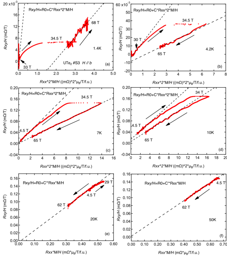
FIG. S8: (color online) R_{xy}/H against R_{xx}^2 M/H at 1.4 K, 4.2 K, 7 K and 10 K. R_{xy}/H against R_{xx} M/H at 20 K and 50 K. The dashed lines are linear fits.
