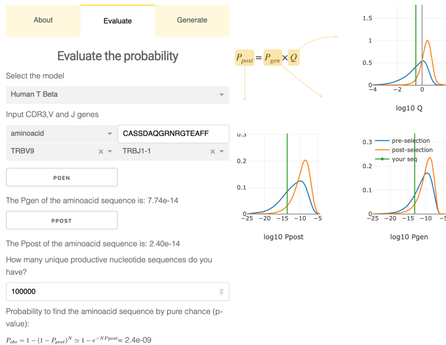
FIG. 1: SOS web interface. The user inputs a CDR3 sequence (amino acid or nucleotides) and V and J segments. The program outputs the generation probability P_{gen} , the probability in the periphery P_{post} , and evaluates a p-value corresponding to the probability of finding that sequence by chance in a repertoire of size N (input by user). An additional tab allows for the generation of synthetic repertoires.
