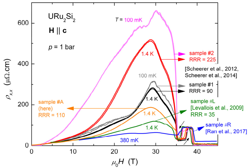
Figure S8. Resistivity \rho versus magnetic field of different samples of \text{URu}_2\text{Si}_2 at low-temperature and in a magnetic field \mathbf{H} \parallel \mathbf{c} . In addition to data from this work, this graph includes data from Refs. [45],[49],[52], [62].
