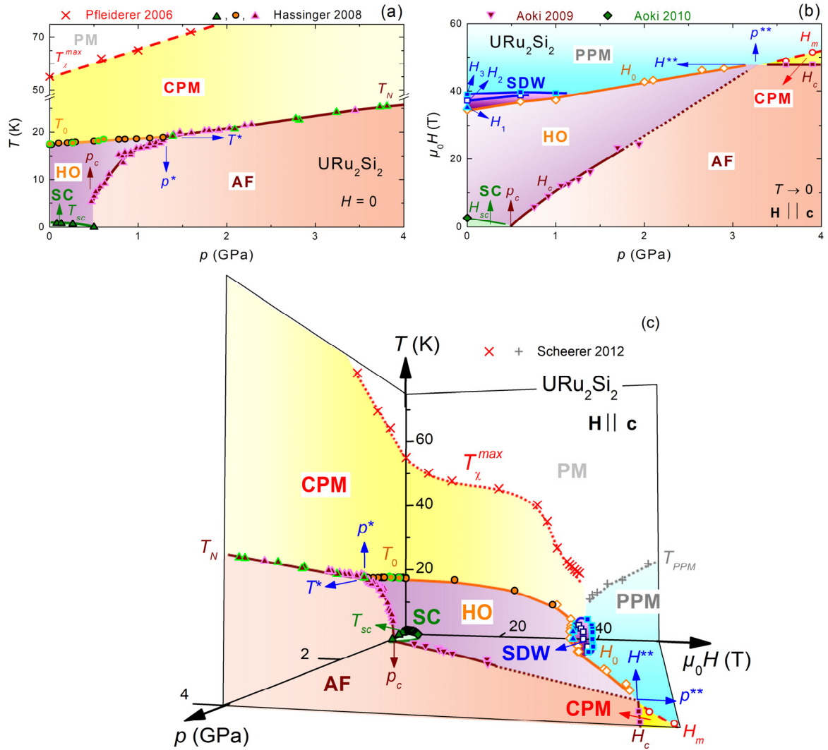
Figure 1. Electronic phase diagram of URu 2 Si 2 under pressure and magnetic field H || c. (a) Temperature – pressure phase diagram at zero field, (b) magnetic field – pressure phase diagram in the limit T \rightarrow 0 , (c) temperature - pressure - magnetic field phase diagram. PM, CPM, and PPM are the high-temperature, the low-temperature correlated, and the high-field polarized paramagnetic regimes, respectively, HO and SC the hidden-order and superconducting phases, respectively, AF the antiferromagnetic state, and SDW the spin-density wave state. In addition to data from this work, data from Refs. [32],[40],[44],[45],[48] (data points from these works and their references are indicated in the Figure) were used to construct these phase diagrams.
