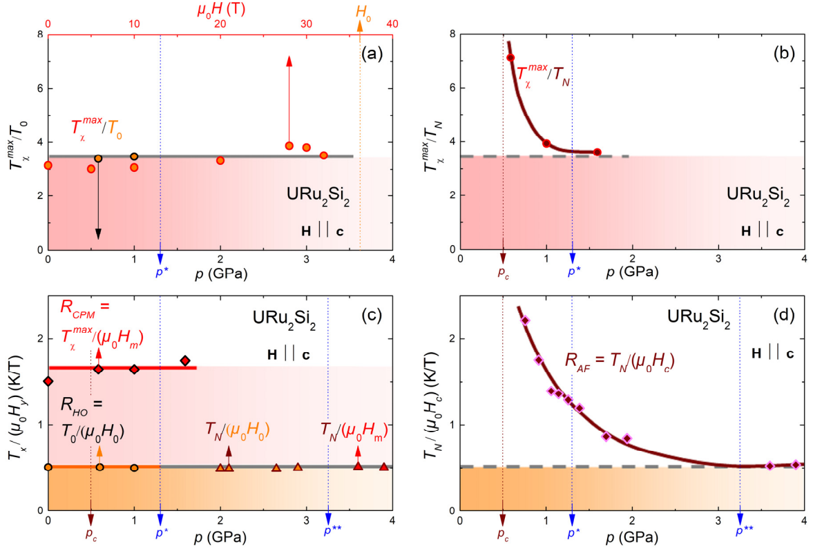
Figure 6. Field- and pressure-variations of characteristic temperature and magnetic-field ratios. Plots of (a) T_\chi^{\max}/T_0 versus H and p , (b) T_\chi^{\max}/T_N versus p , (c) R_{CPM} = T_\chi^{\max}/(\mu_0 H_m) , R_{HO} = T_0/(\mu_0 H_0) , T_N/(\mu_0 H_0) , and T_N/(\mu_0 H_m) versus p , (d) R_{AF} \approx T_N/(\mu_0 H_c) versus p . T_\chi^{\max} is the temperature at which the magnetic susceptibility is maximal. H_m is the metamagnetic field. T_0 and H_0 are the boundaries of the hidden-order phase. T_N and H_c are the boundaries of the antiferromagnetic phase.
