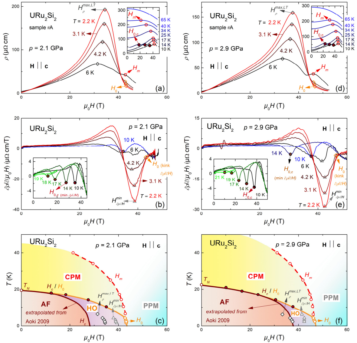
Figure S4. Resistivity \rho and its derivative \partial\rho/\partial H versus magnetic field, and the resulting temperature-magnetic field phase diagrams of \text{URu}_2\text{Si}_2 (sample #A) at the pressures p = 2.1 and 2.9 GPa, in a magnetic field H \parallel c . In addition to data from this work, data extrapolated from Ref. [40] were used to construct these phase diagrams.
