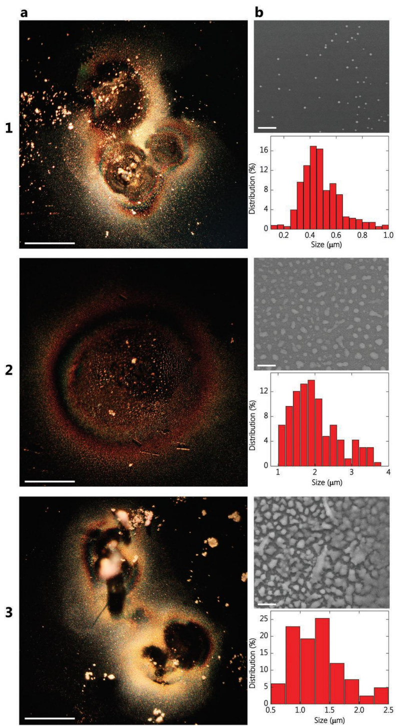
Figure 4. Morphology of MOF derivatives. a) Optical images and b) SEM micrographs and diameter distribution for corresponding derivatives obtained from compounds 1, 2, and 3. Scale bars: a) 50 μm and b) 10 μm for 1 and 2, and 5 μm for 3.
