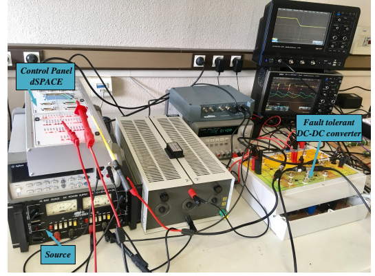
Fig. 7. Fully experimental setup.
