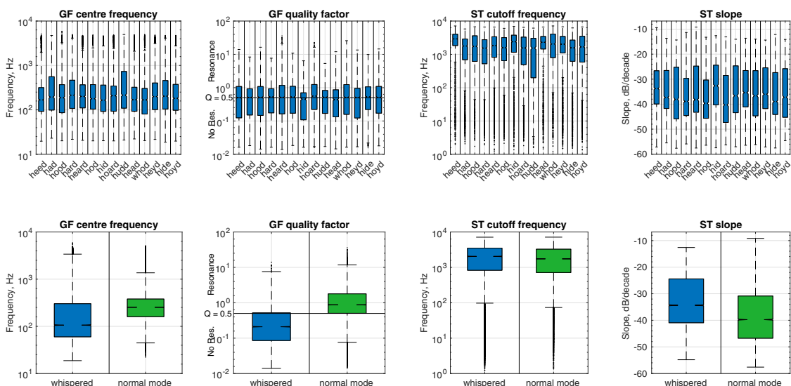
FIGURE 3. Box plots of glottis spectral parameters per vowel (top row) and per phonation mode (bottom row). From left, each row plots the log glottal formant frequency, the log glottal formant quality factor, the log spectral tilt cutoff frequency, and the spectral tilt slope.
