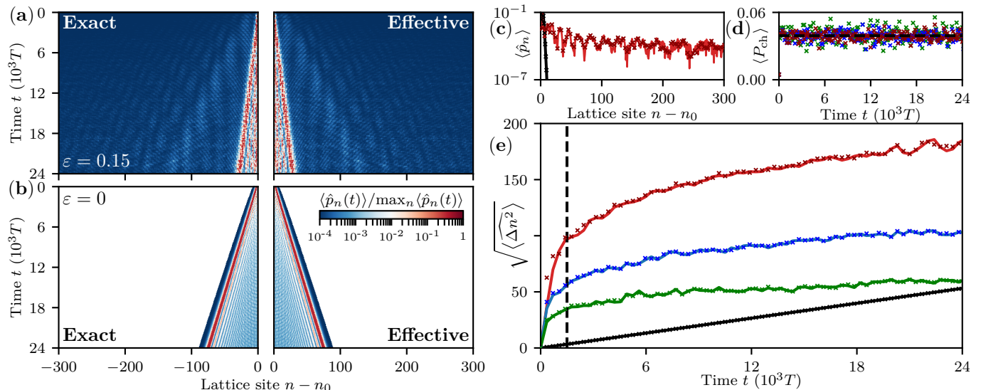
FIG. 3. Dynamics of a wavepacket, initially located on a single regular site n_0 . Parameters are \gamma = 0.2 , \hbar_{\text{eff}} = 0.4 and \varepsilon = 0.15 (modulated lattice) or \varepsilon = 0 (unmodulated lattice). (a-b) Probability at each site vs time, normalized for visibility at each time by its maximum value over the lattice. Exact dynamics in the modulated (a) and unmodulated (b) lattices and its corresponding effective dynamics (note that the system is symmetric through n - n_0 \rightarrow n_0 - n ). (c) Probability at each site for t = 1500T and N = 1079 , solid line for exact dynamics and symbols for effective dynamics, red for \varepsilon = 0.15 and black for \varepsilon = 0 . (d) Overlap of the wavefunction with the chaotic sea in the modulated lattice. Same color code as (c), additional blue ( N = 539 ) and green ( N = 269 ) data for modulated lattices of smaller sizes. (e) Standard deviation of the wavefunction (see text), same color code as (d).
