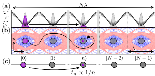
FIG. 1. Equivalent representations of chaos-assisted tunneling in a driven lattice. (a) In situ representation: a wavefunction tunnels through different potential wells. (b) Phase space representation: the wavefunction escapes from an island of stable orbits (blue) by regular tunneling, spreads in the chaotic sea (red) and tunnels in another island. (c) Tight-binding representation: the system is composed of N sites, the coupling between i -th and j -th site is proportional to 1/|i-j| .
