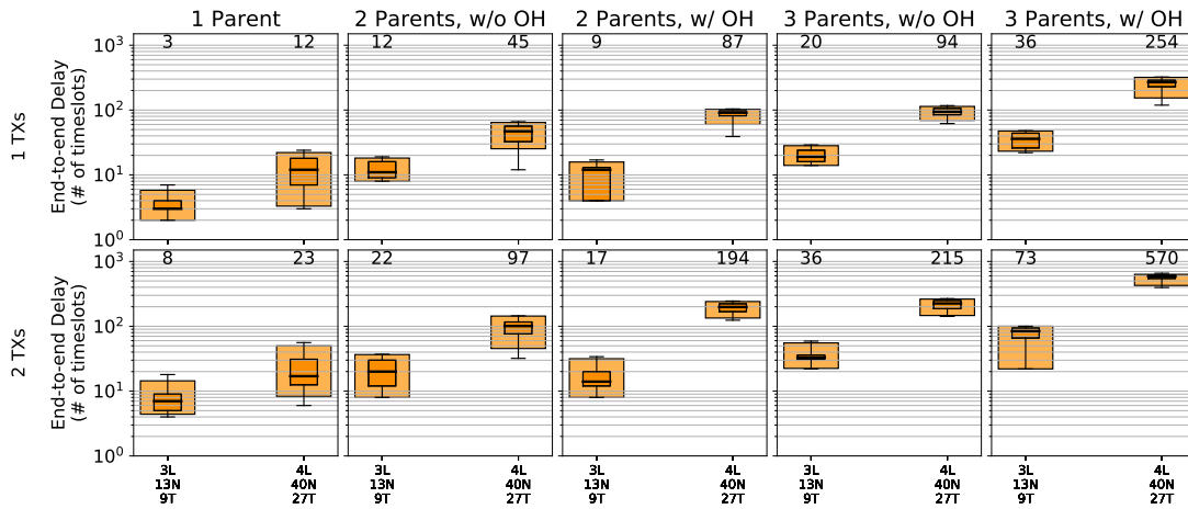
Fig. 12. Results for the end-to-end latency of packets sent from the last layer of the ternary topology. Time in TSCH timeslots, from the first packet TX at the sender, to the last copy RX at the root. In each plot, the outer (lighter) box corresponds to the 5%-95% percentiles, the inner (darker) to the 25%-75% percentiles, the middle line to the median and the whiskers represent the minimum and maximum. On top of each box, the mean value is presented.
