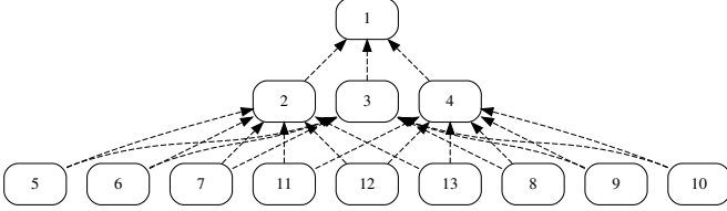
Fig. 6. Ternary-tree-like topology with two parents per node and three layers.
