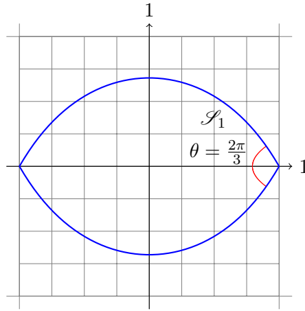
FIGURE 8. The curve \mathcal{S}_1 in (5.10), for the model (5.6) with jumps z = \frac{1}{2} , z_2 = \frac{1}{6} and all other z_r = 0 .
