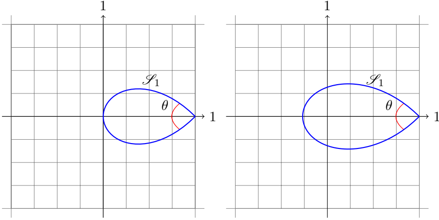
FIGURE 4. The curve \mathcal{S}_1 for the simple walk (left) and for the king walk (right), and definition of the angle \theta . For the two models above, \theta = \frac{\pi}{4} .
