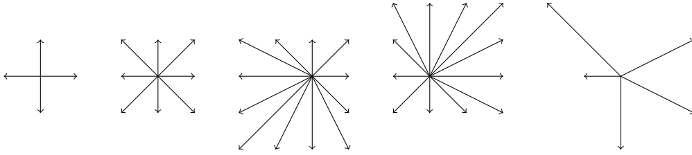
FIGURE 1. Various step sets. From left to right: the simple random walk; the king walk (with jumps to all eight nearest neighbors); an example with big negative jumps; an example with big positive jumps; an arbitrary model.
