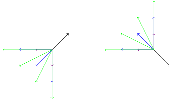
FIGURE 7. On the left: the model studied in Section 5.3. It is inspired by a similar (non-symmetric) model analyzed in [28, 5], displayed on the right picture.
