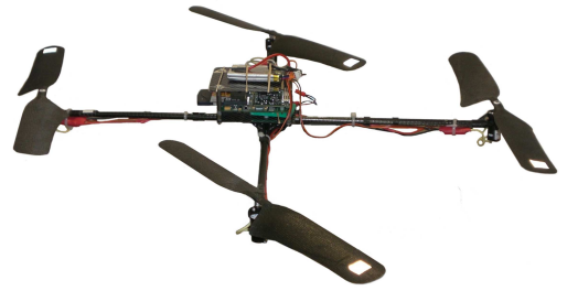
Figure 8. Quadcopter prototype with an highly integrated Inertial Measurement Unit and a ARM-based CPU running a linux OS.
