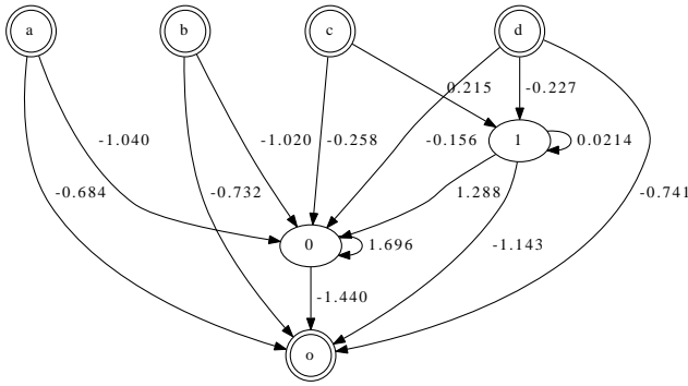
Figure 1: An evolved neural network in the Xor And Xor problem. For each combination of a , b , c and d , the network is simulated during 100 time steps, and if the network is stable, we compare the output o with the expected value of [(a \oplus b) \wedge (c \oplus d)] . If the output is oscillating or unstable, the fitness associated to the network is arbitrarily set to 0. Only connection weights are represented. This network solves the problem with maximum fitness F_x = 1.0 .
