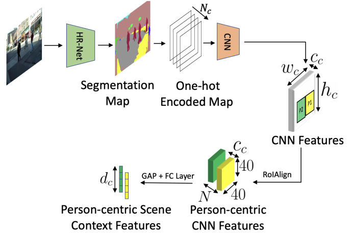
Fig. 7: The scene context network. It encodes nearby scene contextual information of each individual present in a scene. We use this as context network in our proposed model. See III-C for more details.
