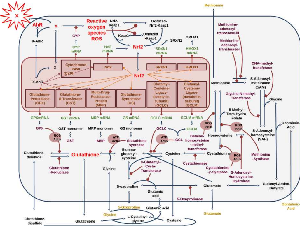
Figure 3: Schematic overview of the assembled SB model. All steps are modeled. This model covers both transcriptional and biochemical aspects of GSH synthesis and metabolism and its control by the Nrf2-Keap1 signaling pathway. The blue compartment is cytosol and the red one is nucleus. Blue arrows show reactant(s):product(s) exchange during biochemical or transport reactions, and red arrows indicate enzymatic catalysis (diamond heads) or gene transcription (round heads). In the nucleus, red boxes represent genes and arrows indicate gene activation. Names of genes are in orange, of mRNA are in green, of enzymes are in purple, of other proteins and metabolites in blue and of extracellular constants in yellow.
